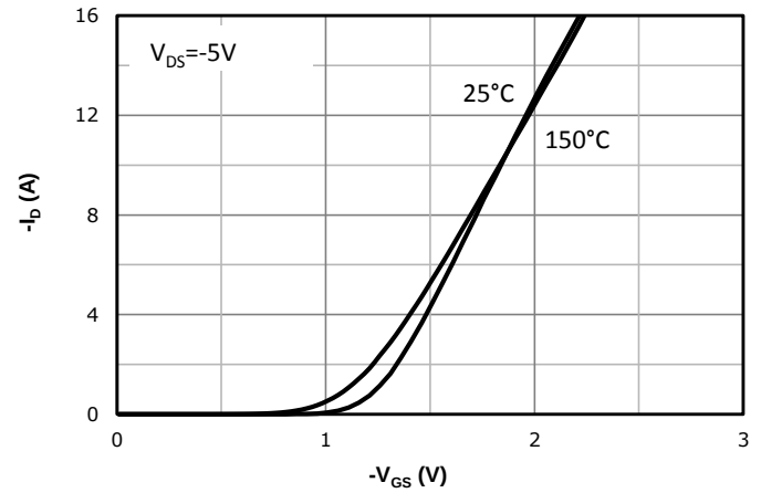
Fig 2: Transfer Characteristics
