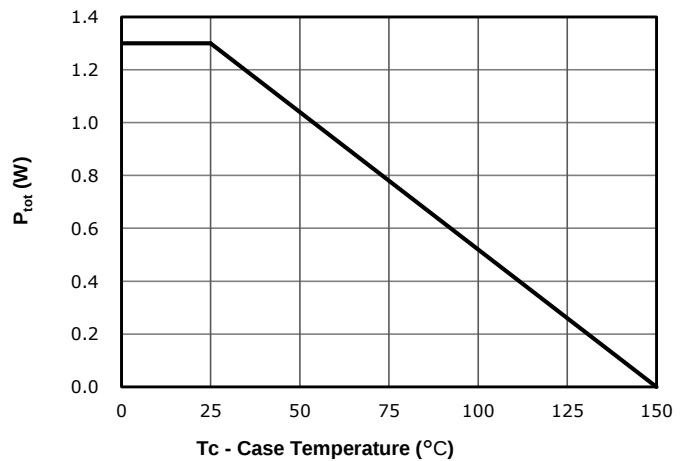
Fig 12: Power Dissipation
