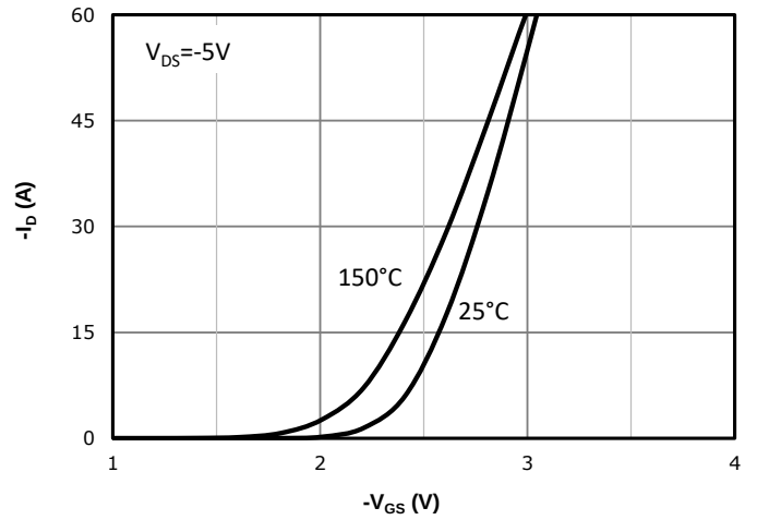
Fig 2: Transfer Characteristics
