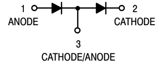
SOT-23 (TO-236) CASE 318 STYLE 11
