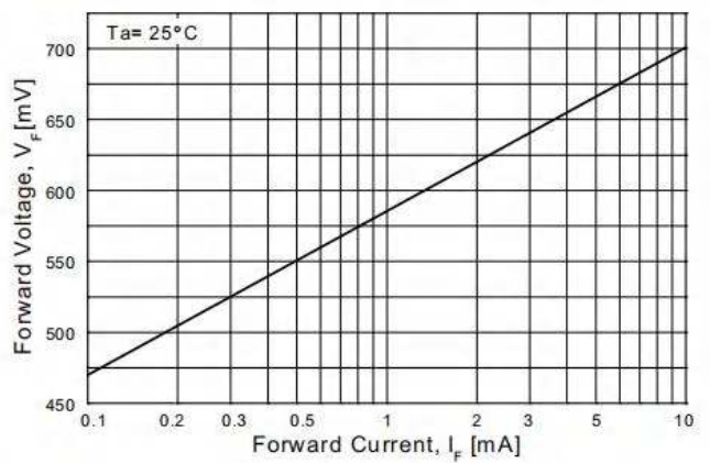
Figure 4. Forward Voltage vs. Forward Current V_F @ I_F = 0.1 to 10 \text{ mA}
