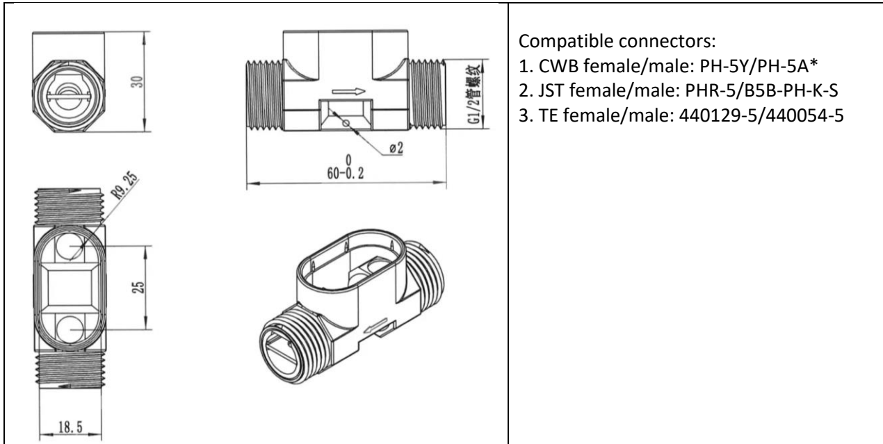
Figure 2: mechanical drawings
