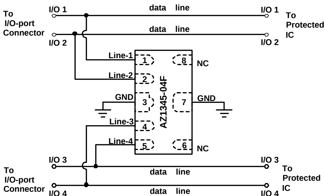
Fig. 1 Data lines connection of AZ1345-04F.
