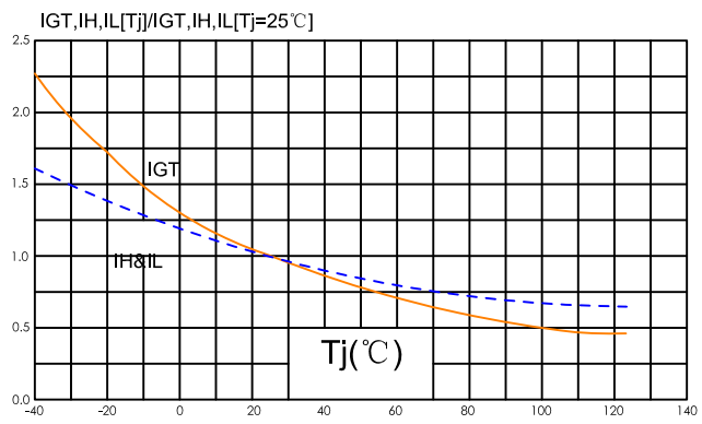
Fig.6: Relative variations of gate trigger current, holding current and latching current versus unjction temperature
