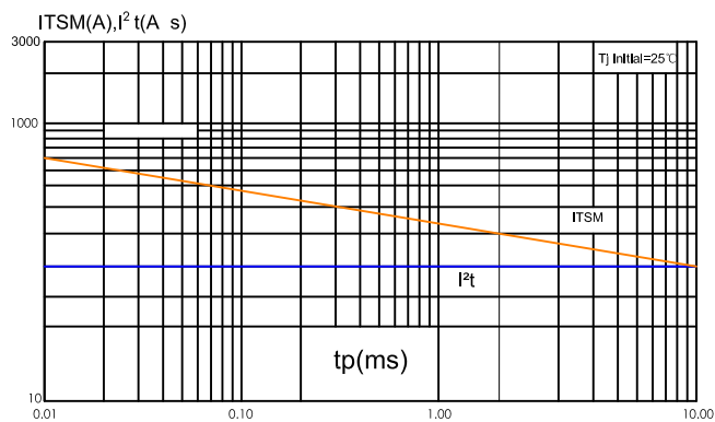
Fig.5 : Non-repetitive surge peak on-state current for a sinusoidal pulse with width t_p < 20\text{ms} and corresponding value of I t ( dI/dt < 100\text{A}/\mu\text{s} )
