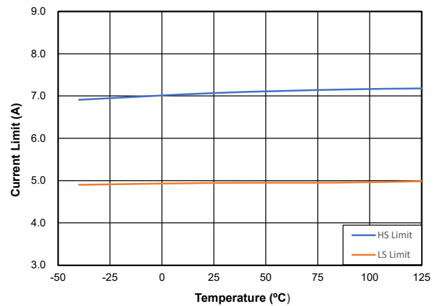
Figure 4. High-Side and Low-Side Current Limits
