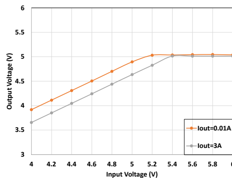
Figure 11. Low Drop-out Voltage
