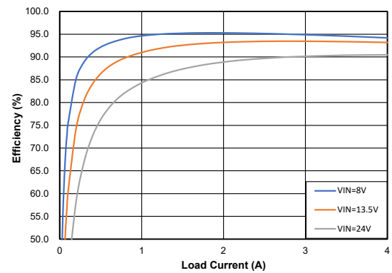
Figure 16. Efficiency
