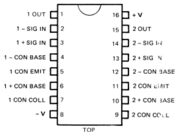
Pin Diagram
