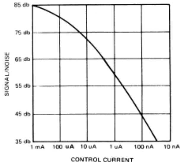
Signal Noise vs Control Current (6 Vpp in)
