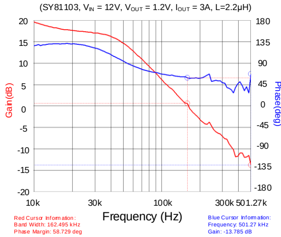
Bode Plot
