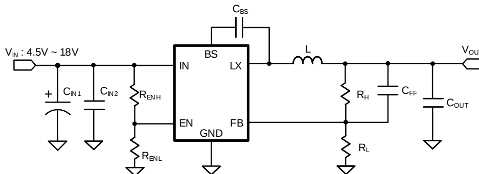
Figure9. Schematic Diagram
