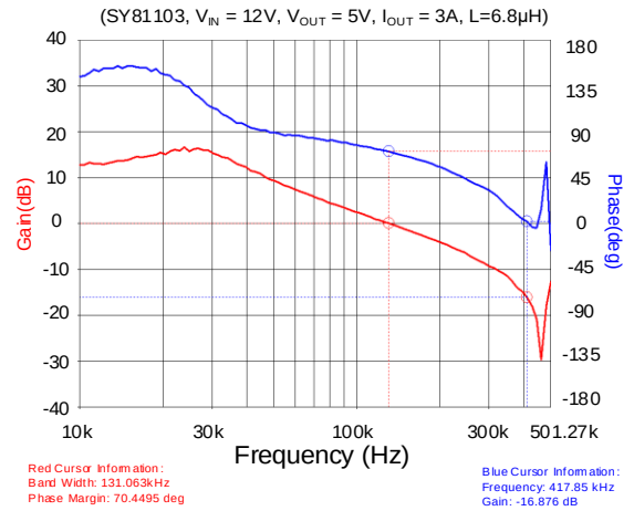
Bode Plot
