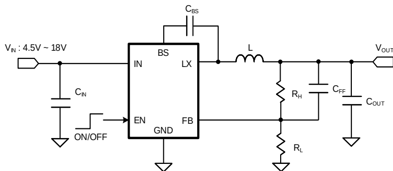
Figure1. Schematic Diagram
