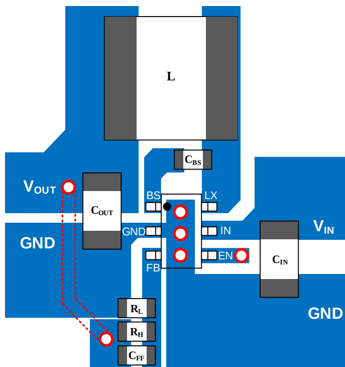
Figure10. Suggested PCB Layout
