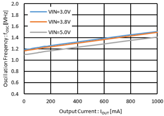
XC9285, V_{OUT(T)}=3.3V
