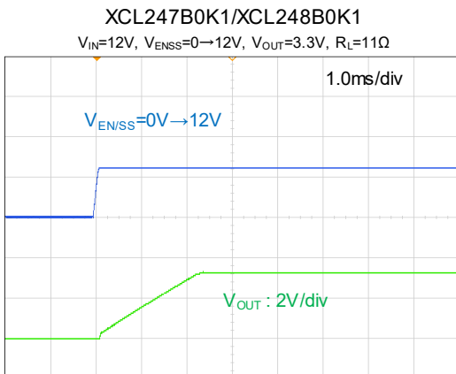
(19) Start-up Waveform (EN/SS Rising)
