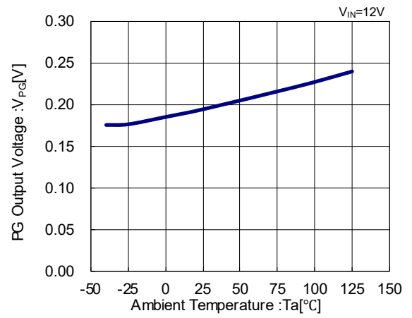
(15) PG Output Voltage vs. Ambient Temperature
