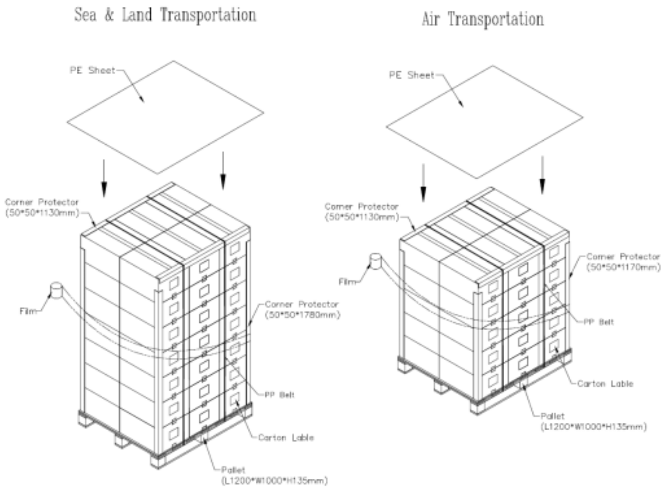
Figure. 7-3 Packing method
