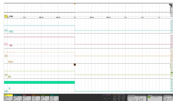
Figure 34. Power down by Enable
