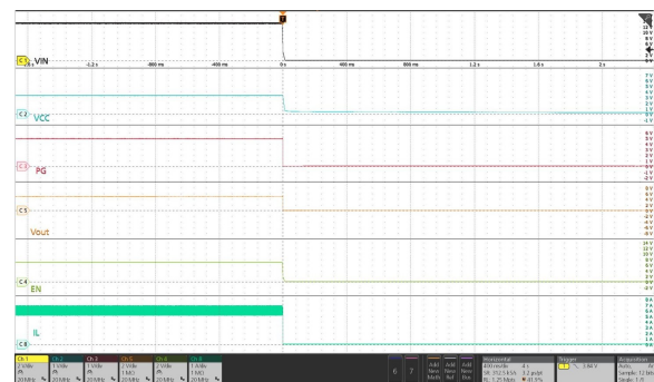
Figure 30. Power down by Inputs
