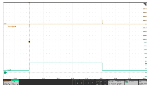
Figure 24. Load Transient
