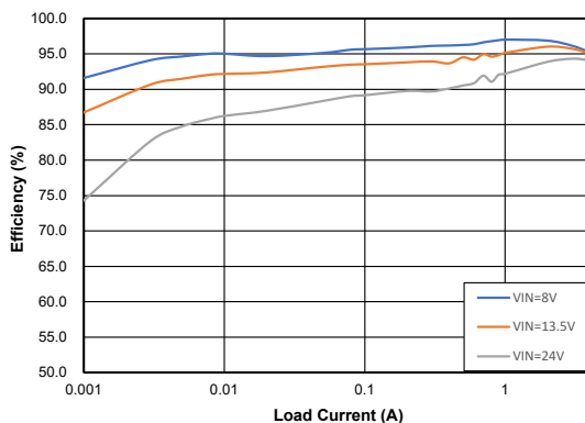
Figure 13. Efficiency
