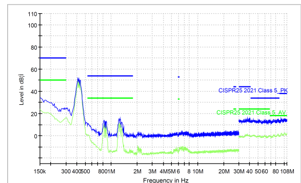
Figure 36. Power down by Enable
