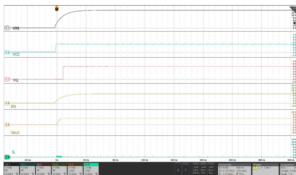
Figure 27. Short Circuit Protection
