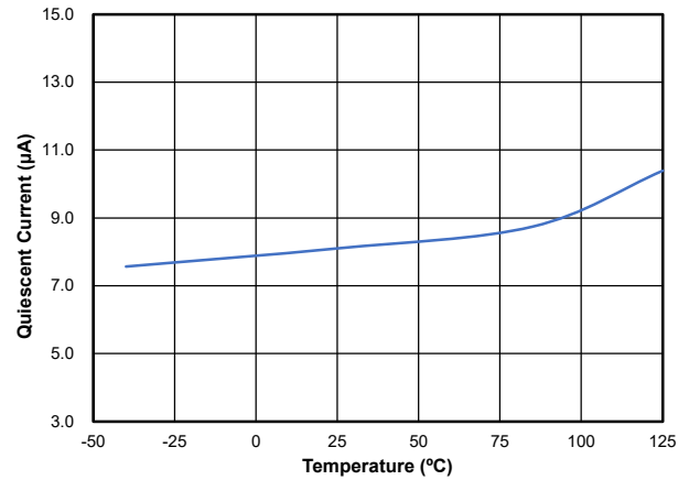
Figure 2. Quiescent Current
