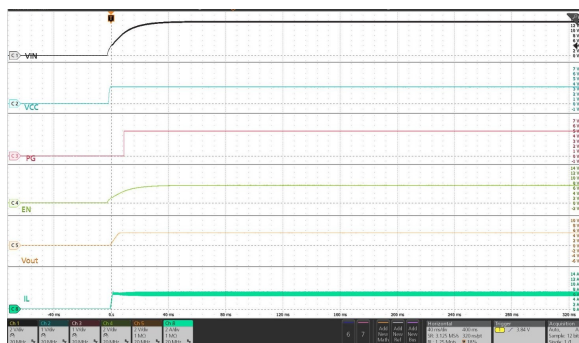
Figure 29. Power up by Inputs
