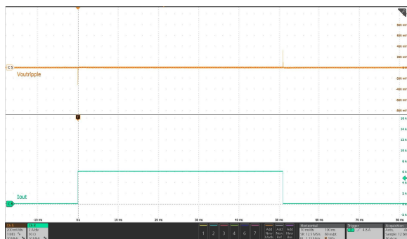
Figure 23. Load Transient
