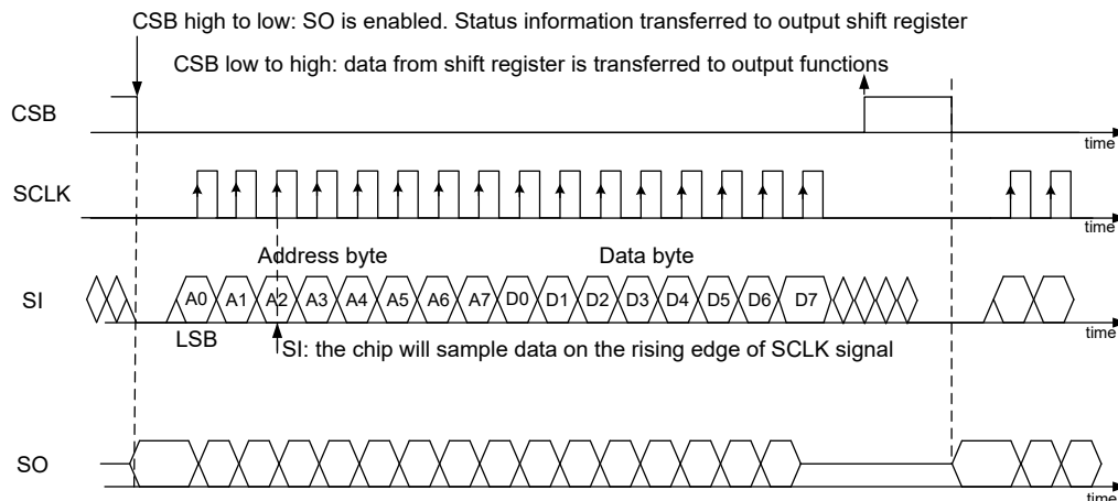
Figure 9. SI Data Transfer Timing
