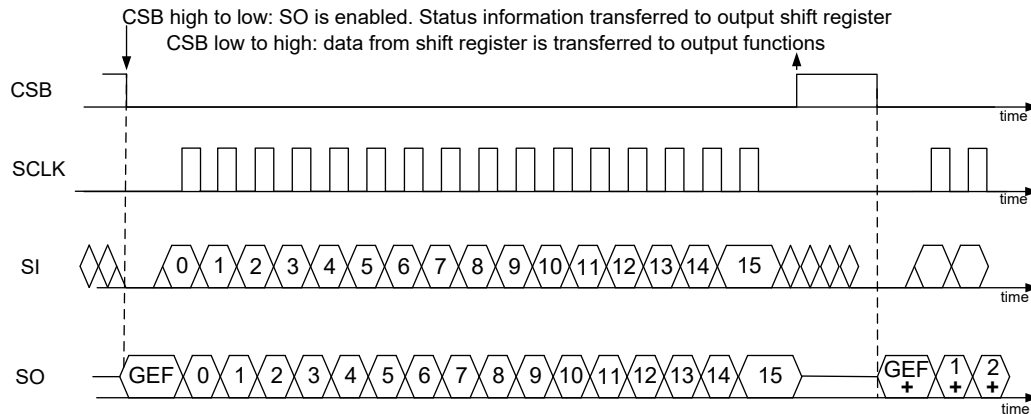
Figure 8. SPI Timing
