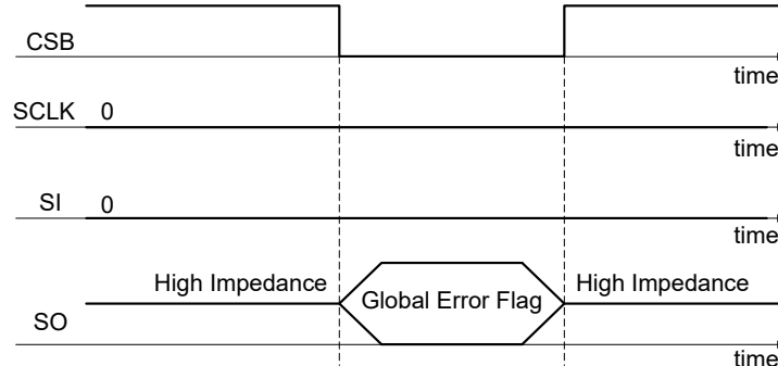
Figure 12. SO Behavior with 0-clock Cycle
