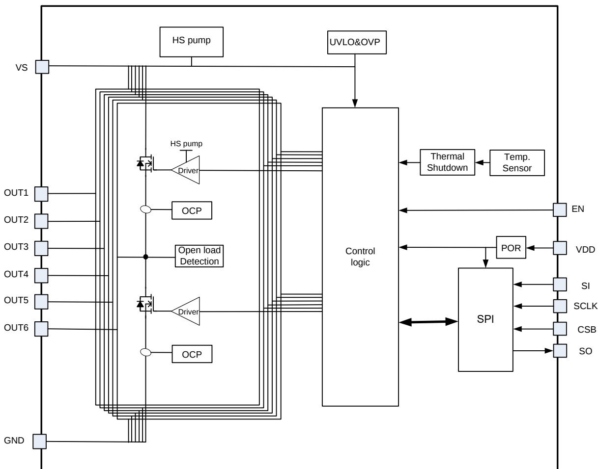
Figure3. SY2A58119 Block Diagram
