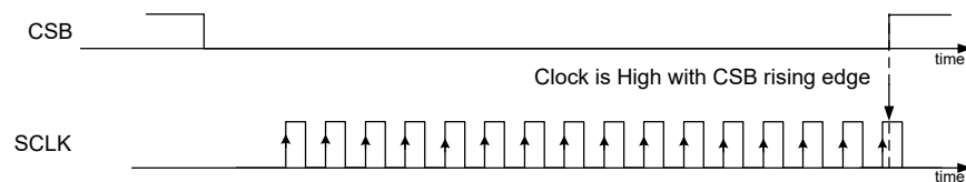
Figure13. Clock Polarity Error
