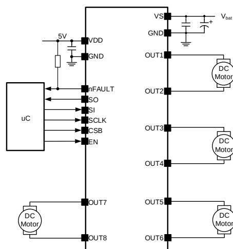
Figure 1. Typical Application Circuit
