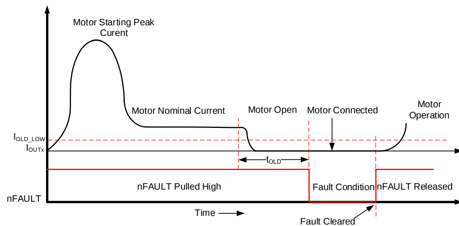
Figure 17. Low-current OLD
