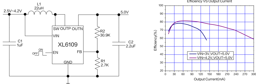
Figure4. XL6109 System Application and efficiency curve ( V_{OUT}=5.0V )
