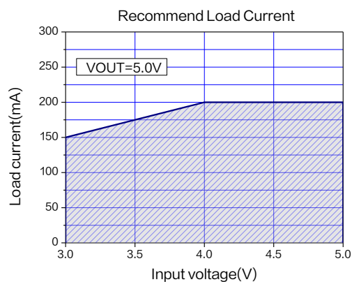
Figure 12.Max Output Current ( V_{OUT}=5.0V , T_A=25^{\circ}C )
