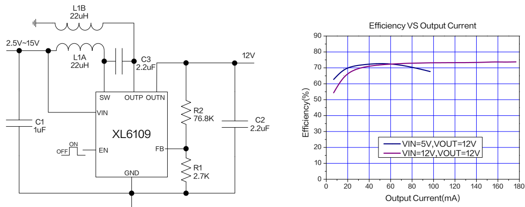
Figure7. XL6109 System Application and efficiency curve( V_{IN}=2.5V\sim15V, V_{OUT}=12V )
