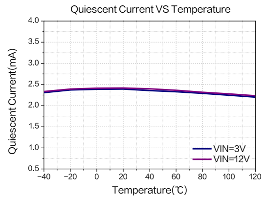
Figure 11.Quiescent Current
