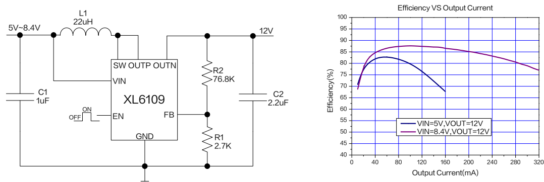
Figure5. XL6109 System Application and efficiency curve ( V_{OUT}=12V )
