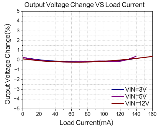
Figure 9. Load Regulation
