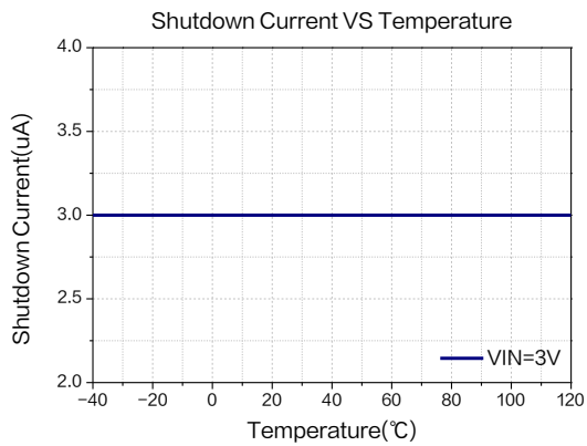
Figure 10.Shutdown Current
