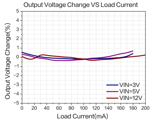
Figure 9. Load Regulation
