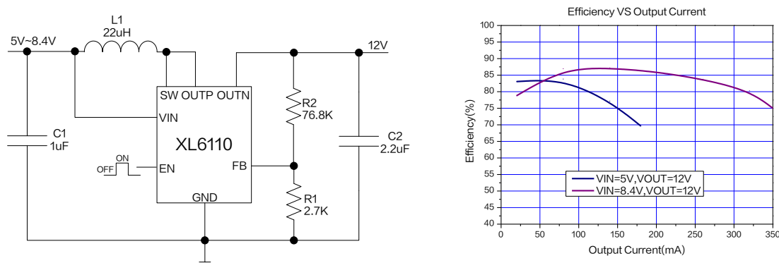
Figure5. XL6110 System Application and efficiency curve ( V_{OUT}=12V )
