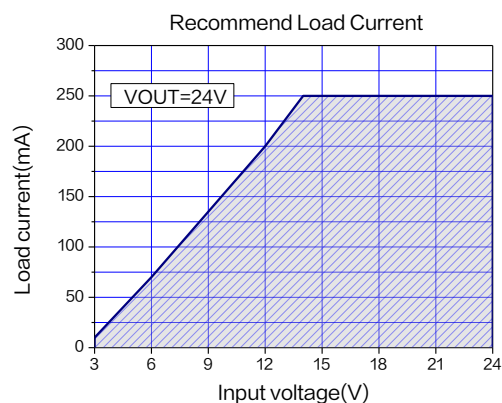
Figure 15.Max Output Current ( V_{OUT}=24V , T_A=25^{\circ}C )
