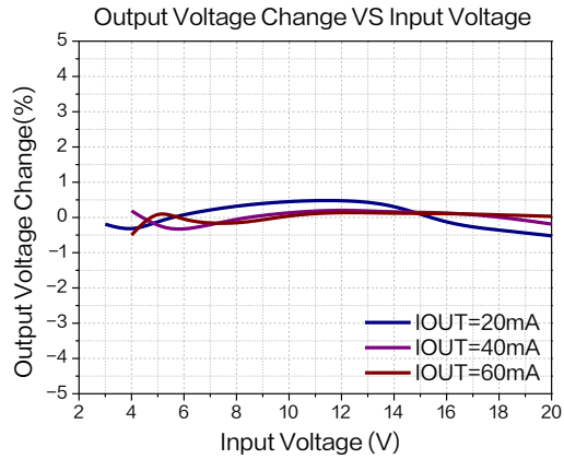
Figure 8.Line Regulation
