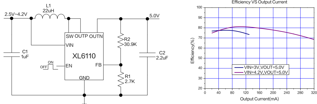
Figure4. XL6110 System Application and efficiency curve ( V_{OUT}=5.0V )
