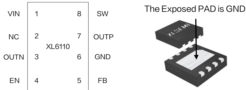
Figure2. Pin Configuration of XL6110
