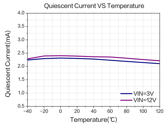
Figure 11.Quiescent Current
