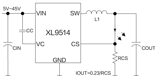
Figure1. XL9514 Typical application schematic and efficiency curve
