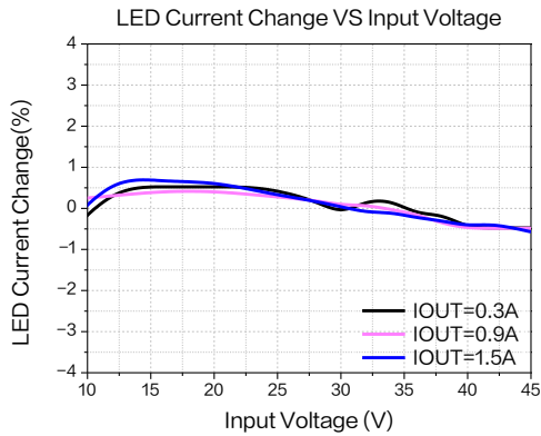
Figure13.Line Regulation
