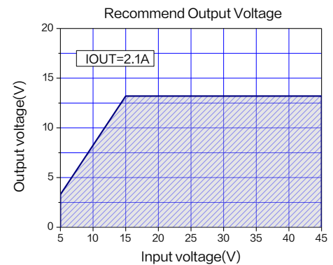
Figure20.Max Output Voltage ( I_{OUT}=2.1A , T_A=25^{\circ}C )
