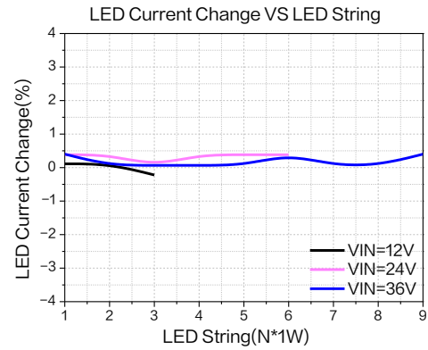
Figure14.Load Regulation
