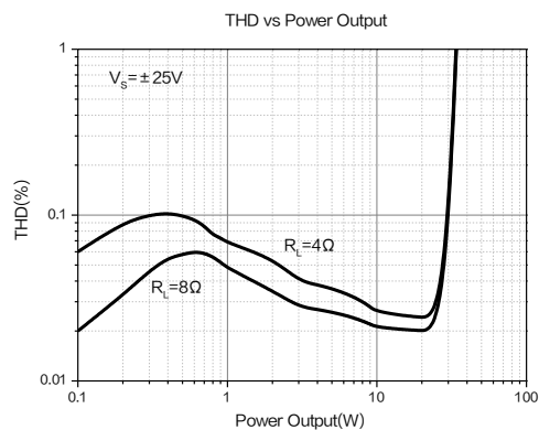
Figure 5. THD vs Power Output
