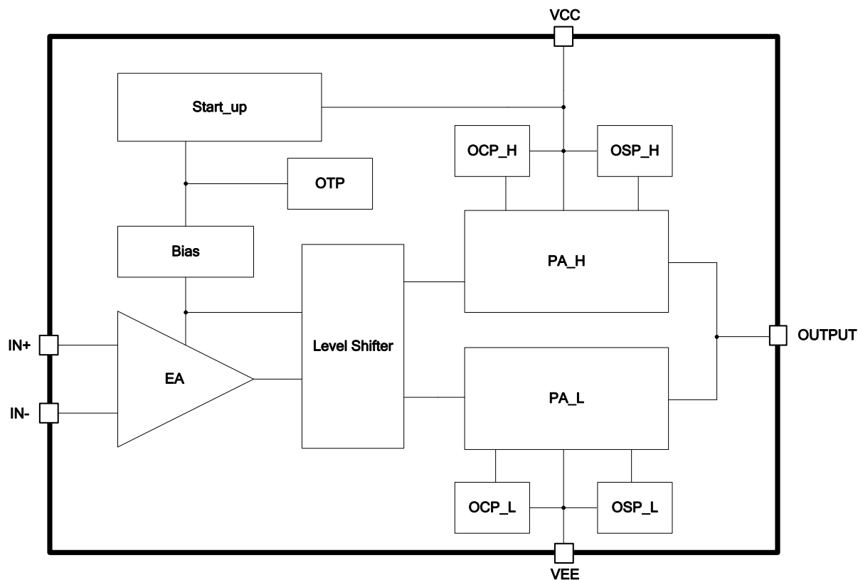
Figure3.Function Block Diagram of XL1875
