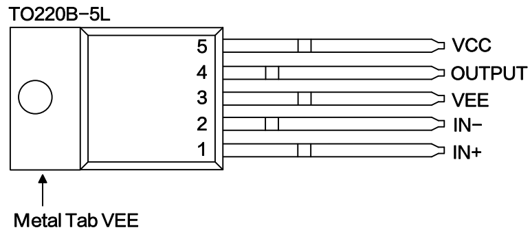
Figure2.Pin Configuration of XL1875
