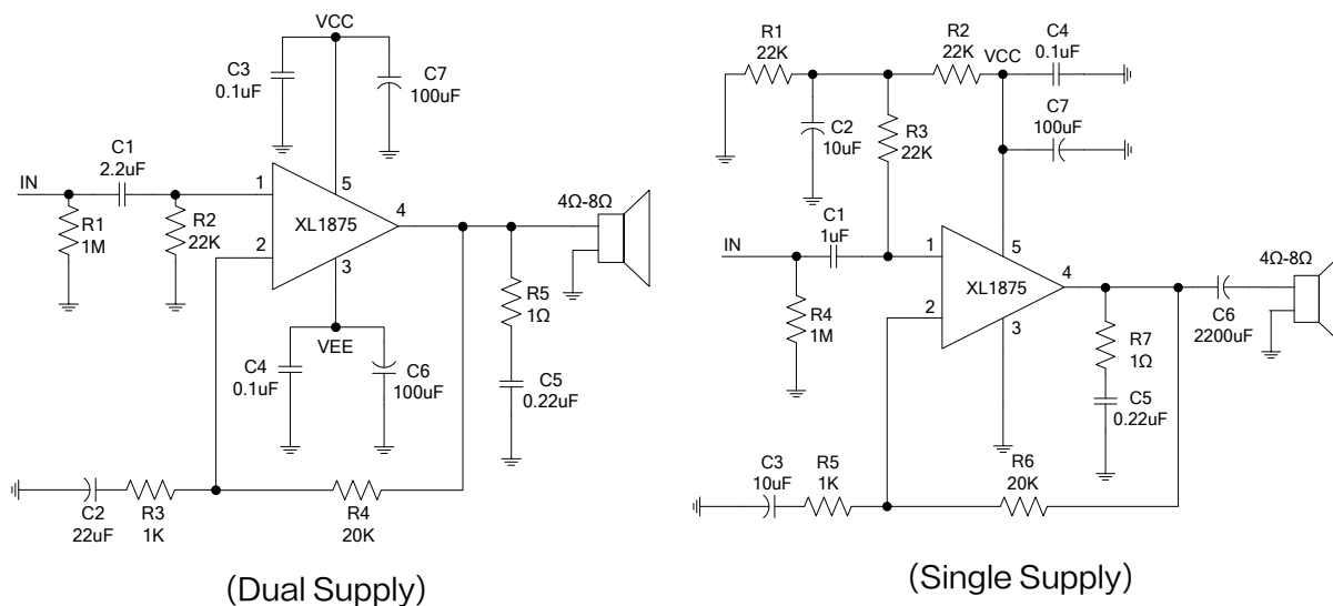
Figure 4.XL1875 Typical Application Circuit
