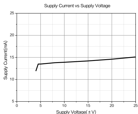
Figure 8. Quiescent Current
