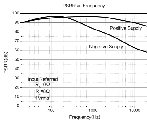
Figure 9.PSRR vs Frequency
