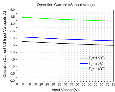
Figure6.Operation Current
