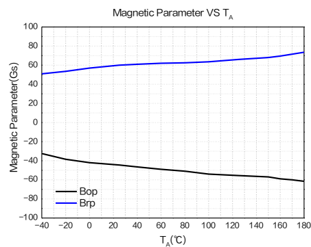
Figure8.Magnetic Operating Point VS Temperature Curve
