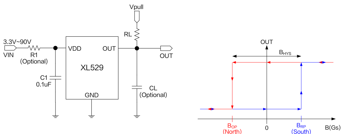
Figure1.XL529 Typical application schematic and output characteristic curve
