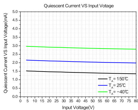
Figure5.Quiescent Current
