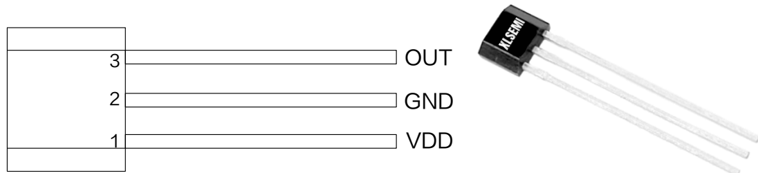
Figure2.Pin Configuration of XL529
