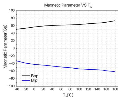
Figure8.Magnetic Operating Point VS Temperature Curve
