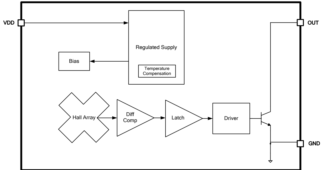
Figure3.Function Block Diagram of XL533
