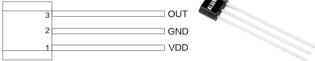
Figure2.Pin Configuration of XL533
