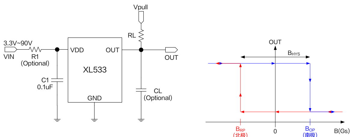
Figure1.XL533 Typical application schematic and output characteristic curve
