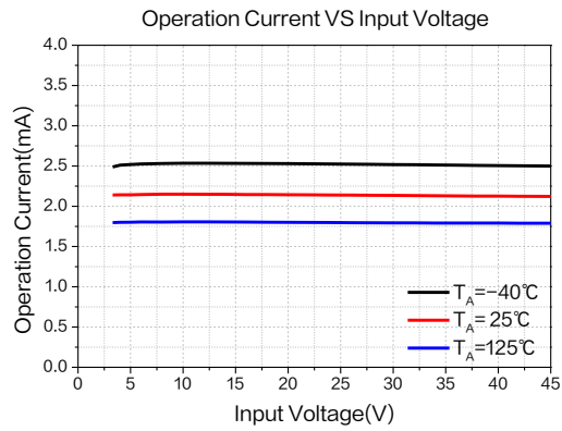
Figure 5. Operation Current
