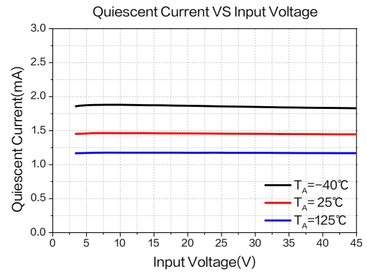
Figure 6. Quiescent Current
