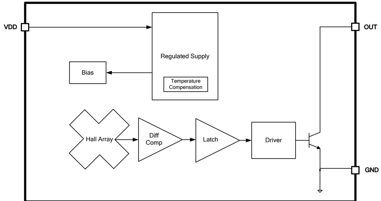
Figure3. Function Block Diagram of XL557
