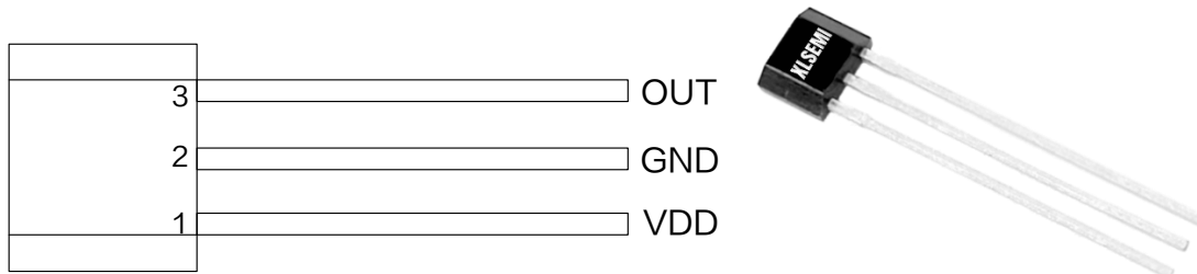
Figure2. Pin Configuration of XL557
