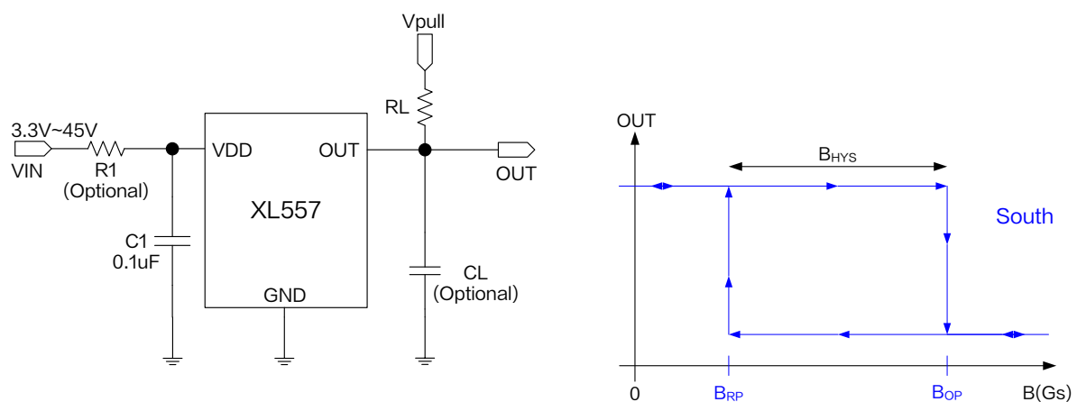
Figure1. XL557 Typical application schematic and output characteristic curve
