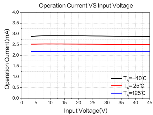
Figure 5.Operation Current
