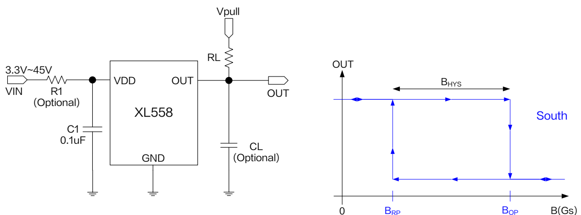
Figure1. XL558 Typical application schematic and output characteristic curve
