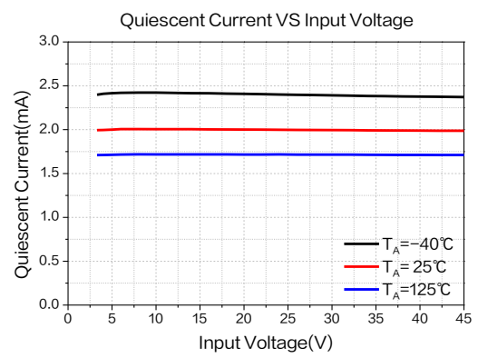
Figure 6.Quiescent Current
