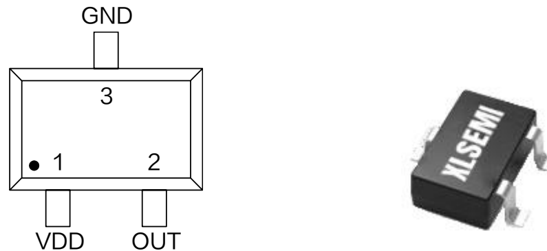
Figure2. Pin Configuration of XL558
