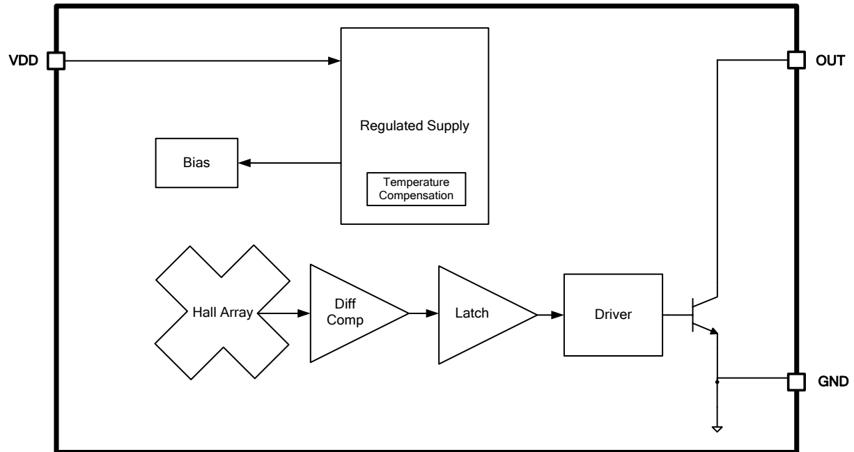
Figure3. Function Block Diagram of XL558
