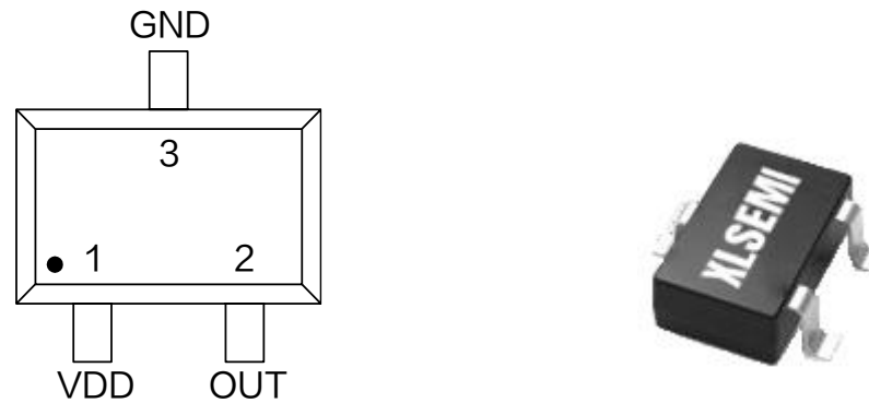
Figure2. Pin Configuration of XL566
