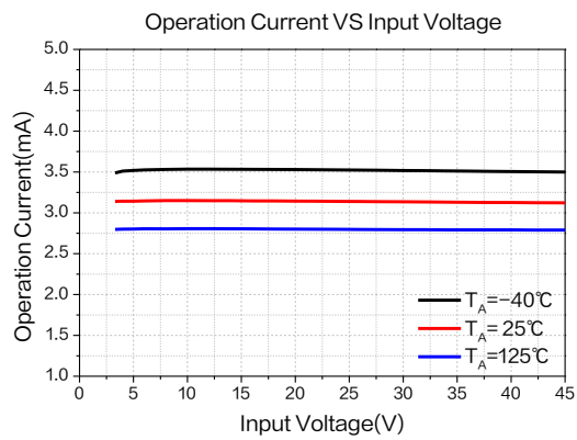
Figure 5. Operation Current
