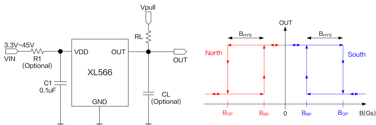
Figure1. XL566 Typical application schematic and output characteristic curve
