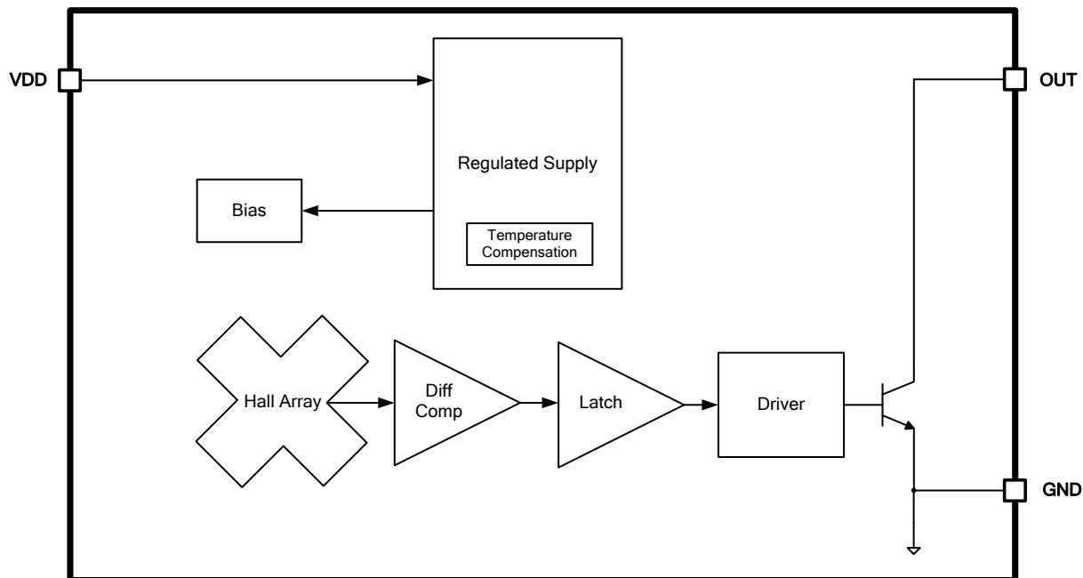
Figure3. Function Block Diagram of XL566
