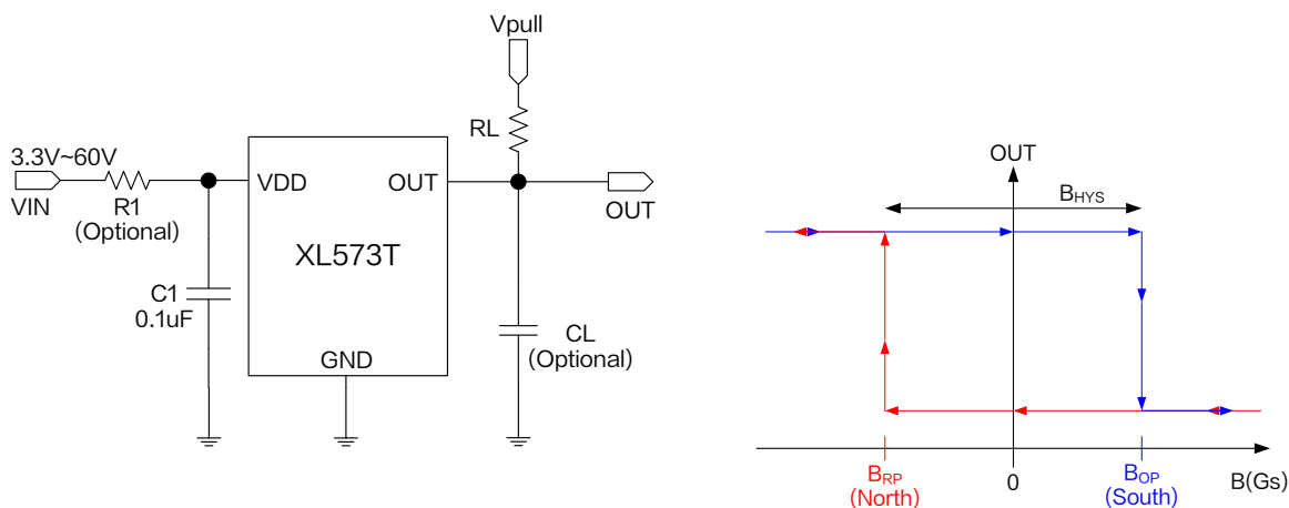
Figure1.XL573T Typical application schematic and output characteristic curve
