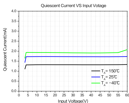
Figure5.Quiescent Current
