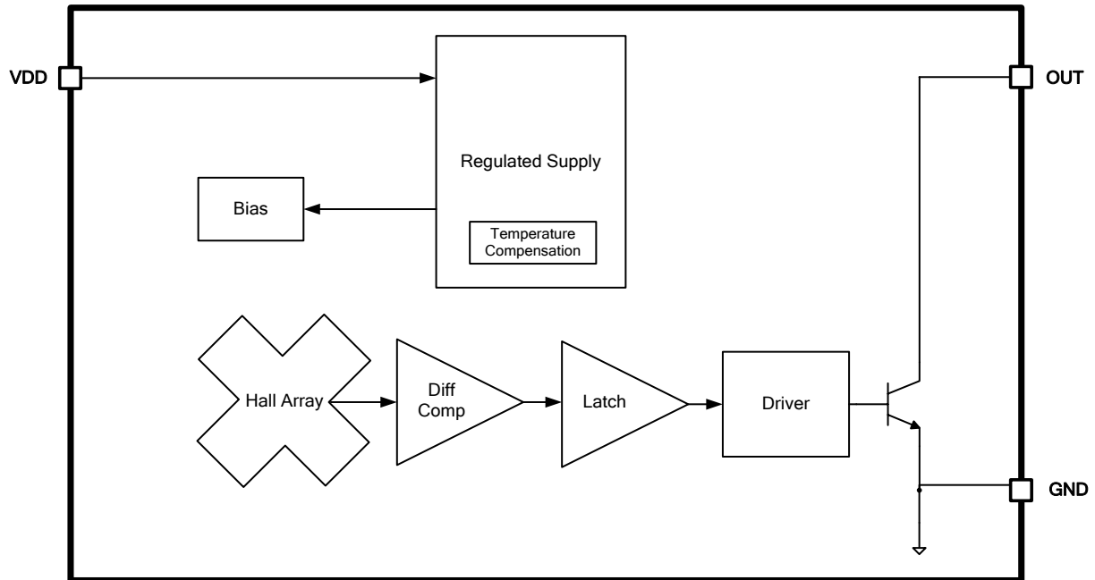
Figure3.Function Block Diagram of XL573T
