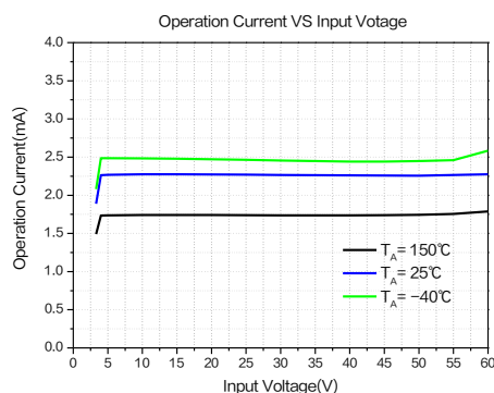
Figure6.Operation Current
