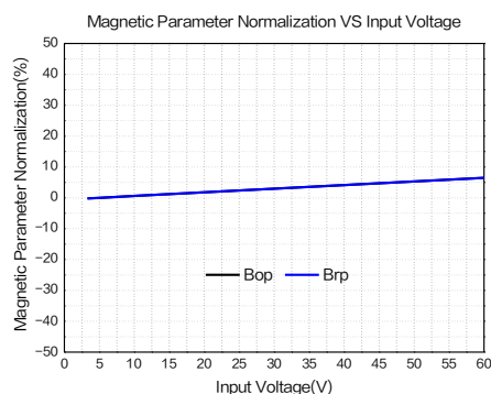
Figure9.Magnetic Operating Point VS Input Voltage Curve
