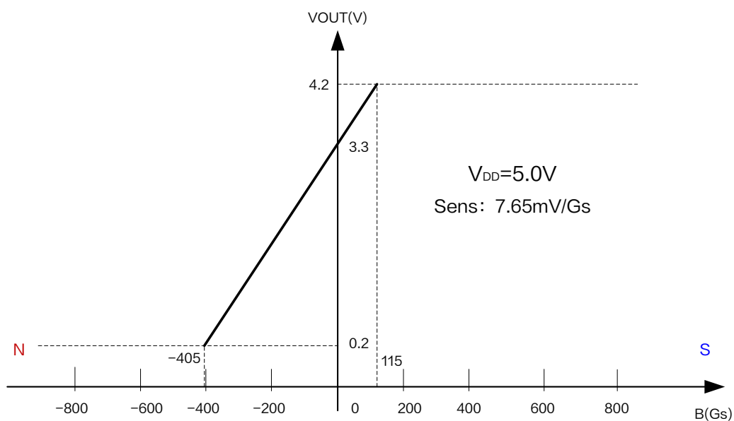
Figure6.XL42N Output characteristic curve ( V_{DD} = 5.0V )
