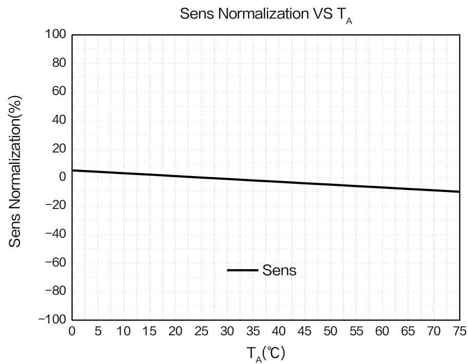
Figure7.Sensitivity versus temperature curve of XL42N ( V_{DD} = 3.3V )
