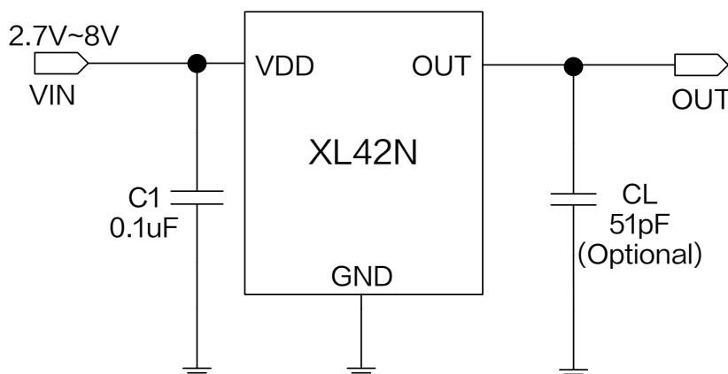
Figure1.XL42N Typical application schematic
