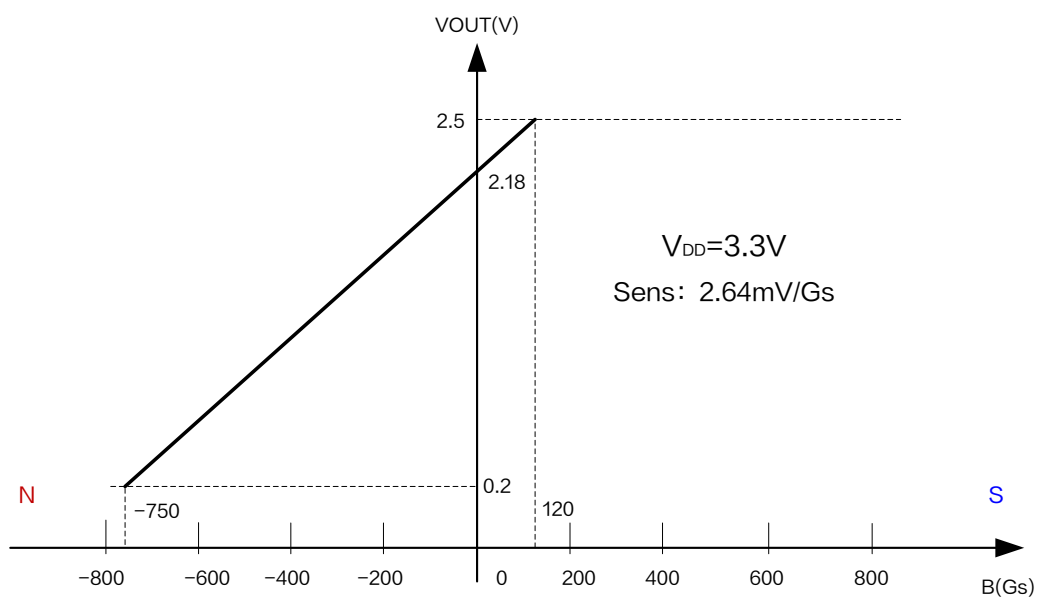
Figure5.XL42N Output characteristic curve ( V_{DD} = 3.3V )
