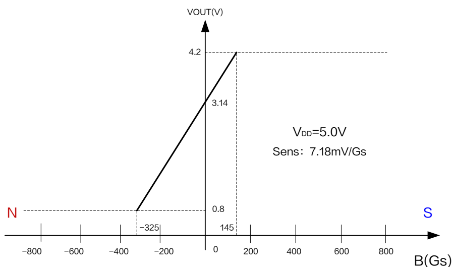
Figure6.Output characteristic curve of XL41 ( V_{DD}=5.0V )
