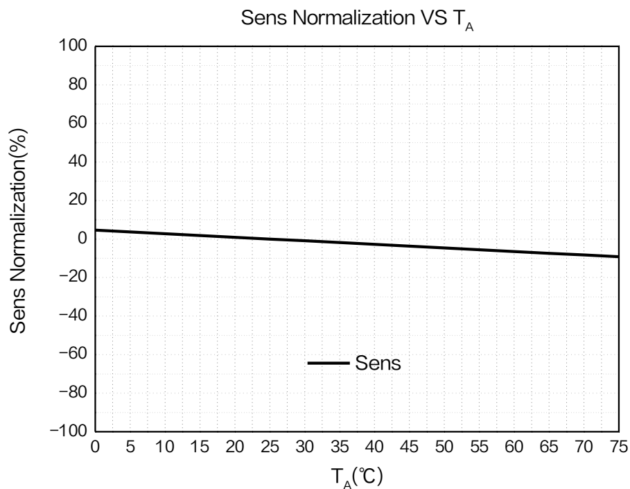
Figure7.Sensitivity versus temperature curve of XL41 ( V_{DD}=3.3V )
