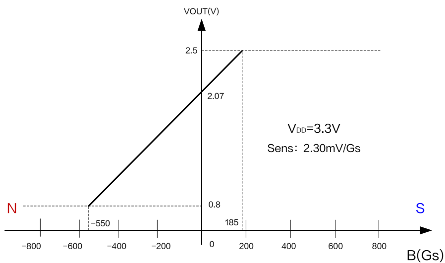
Figure5.Output characteristic curve of XL41 ( V_{DD}=3.3\text{V} )
