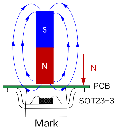
Figure4.Application diagram of XL41
