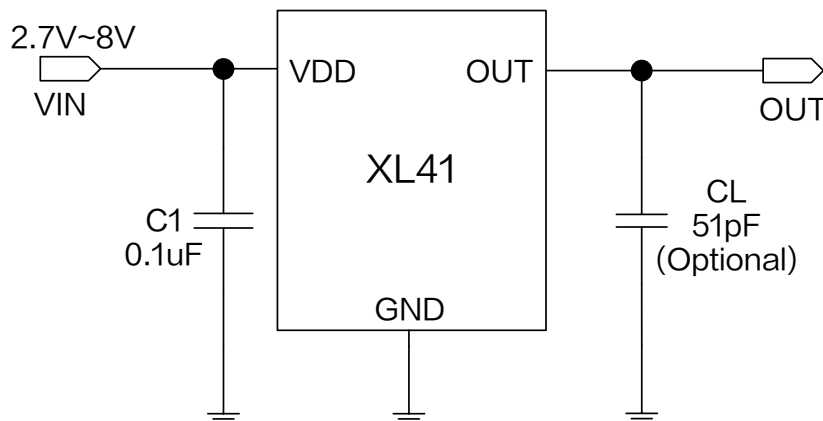
Figure1.XL41 Typical application schematic
