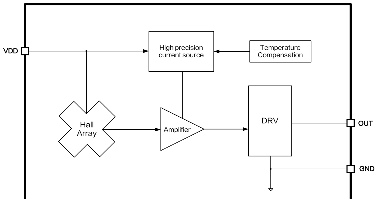
Figure3.Function Block Diagram of XL41
