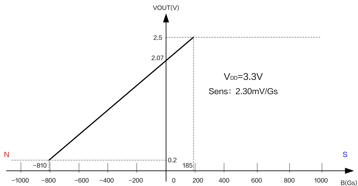
Figure5.XL42W Output characteristic curve ( V_{DD} = 3.3V )
