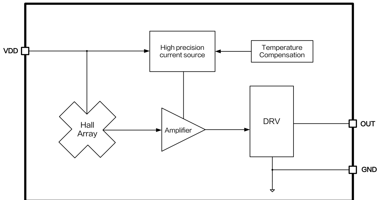
Figure3.Function Block Diagram of XL42W
