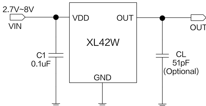
Figure1.XL42W Typical application schematic
