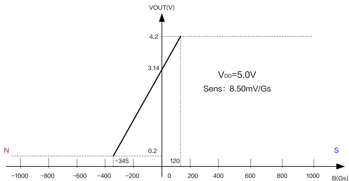
Figure6.XL42W Output characteristic curve ( V_{DD} = 5.0V )
