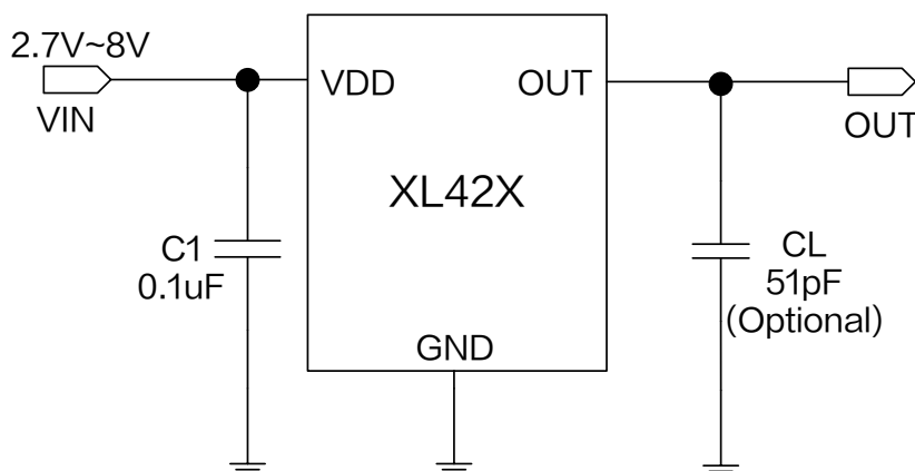
Figure1.XL42X Typical application schematic
