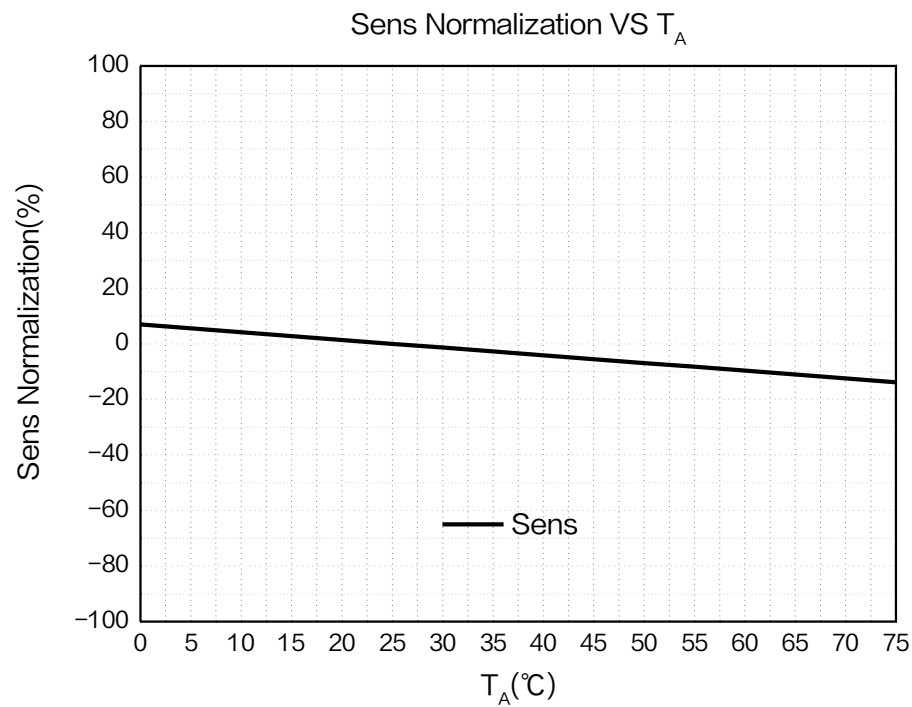
Figure7. Sensitivity versus temperature curve of XL42X ( V_{DD}=3.3V )
