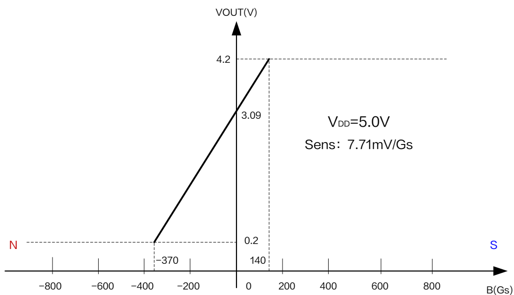
Figure6.XL42X Output characteristic curve ( V_{DD}=5.0V )
