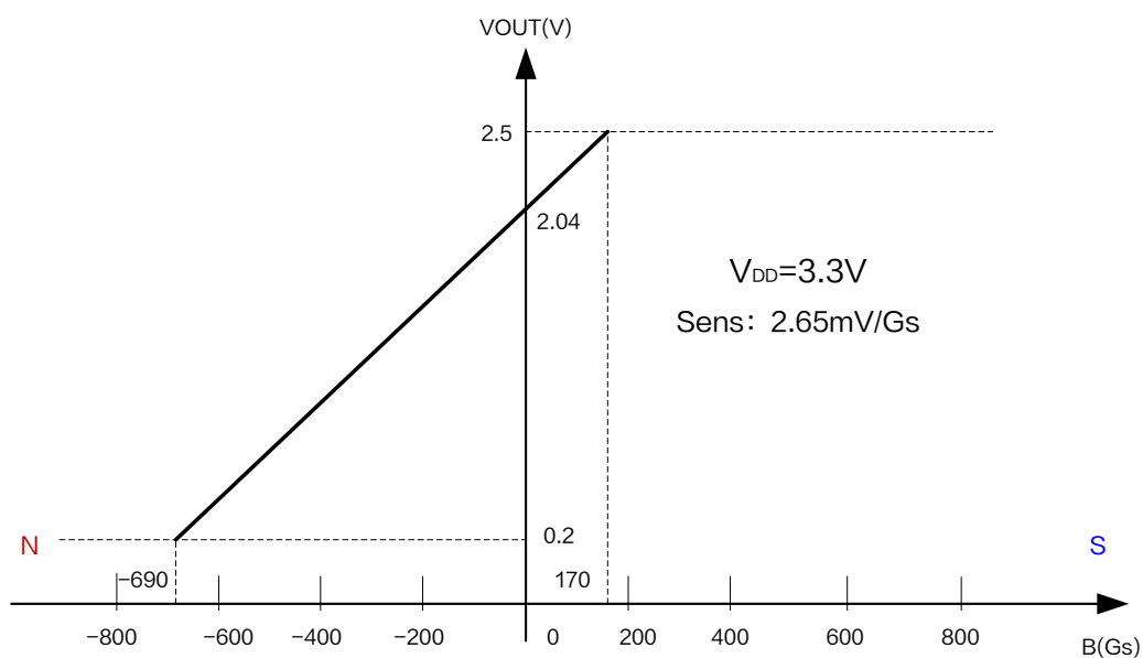
Figure5.XL42X Output characteristic curve ( V_{DD}=3.3V )
