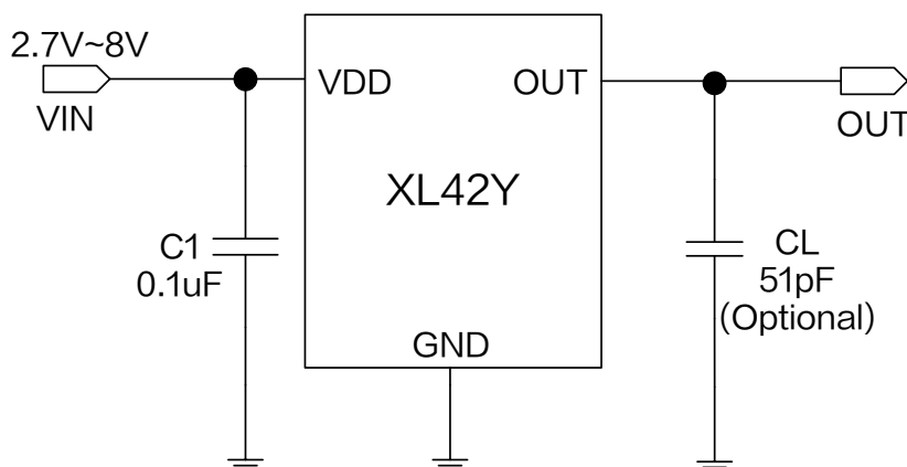
Figure1.XL42Y Typical application schematic
