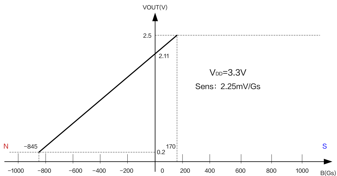
Figure5.XL42Y Output characteristic curve ( V_{DD} = 3.3V )
