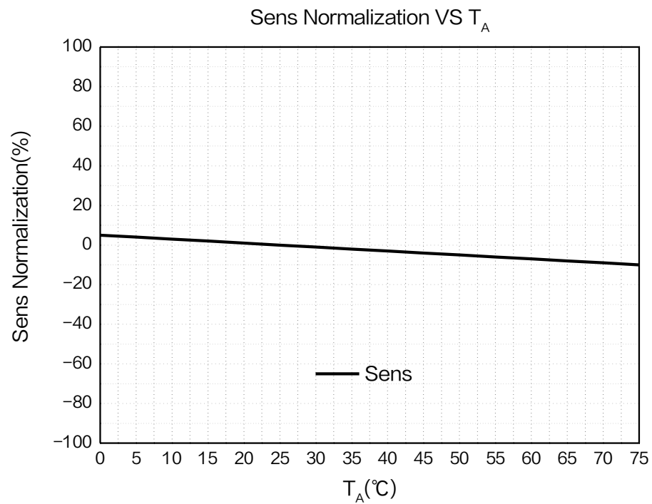
Figure7.Sensitivity versus temperature curve of XL42Y ( V_{DD} = 3.3V )
