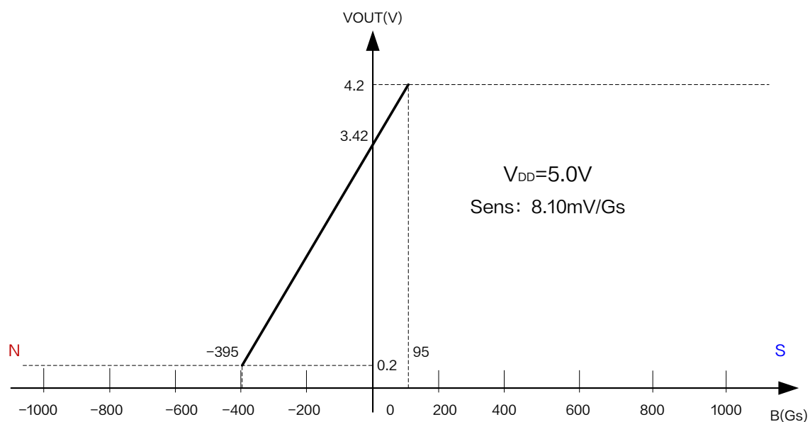
Figure6.XL42Y Output characteristic curve ( V_{DD} = 5.0V )
