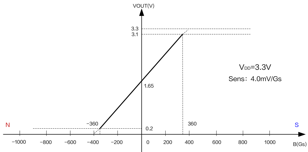
Figure5.Output Characteristic Curve of XL44A ( V_{DD} = 3.3V )
