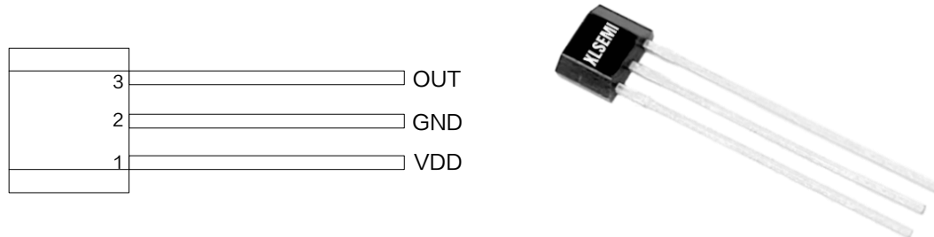
Figure2.Pin Configuration of XL44A
