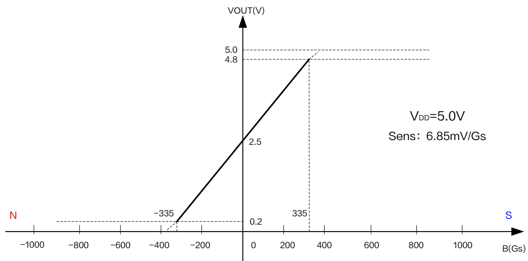
Figure6.Output Characteristic Curve of XL44A ( V_{DD} = 5.0V )
