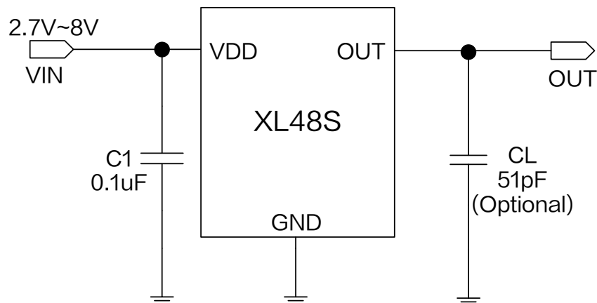
Figure1.XL48S Typical application schematic
