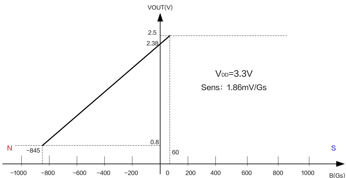
Figure5.XL48S Output characteristic curve ( V_{DD} = 3.3V )
