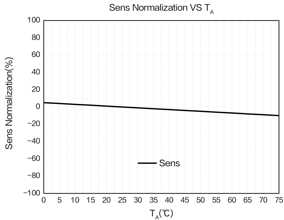
Figure7. Sensitivity versus temperature curve of XL48S ( V_{DD} = 3.3V )
