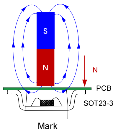
Figure4. Application diagram of XL48S
