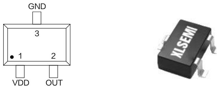
Figure2.Pin Configuration of XL48S
