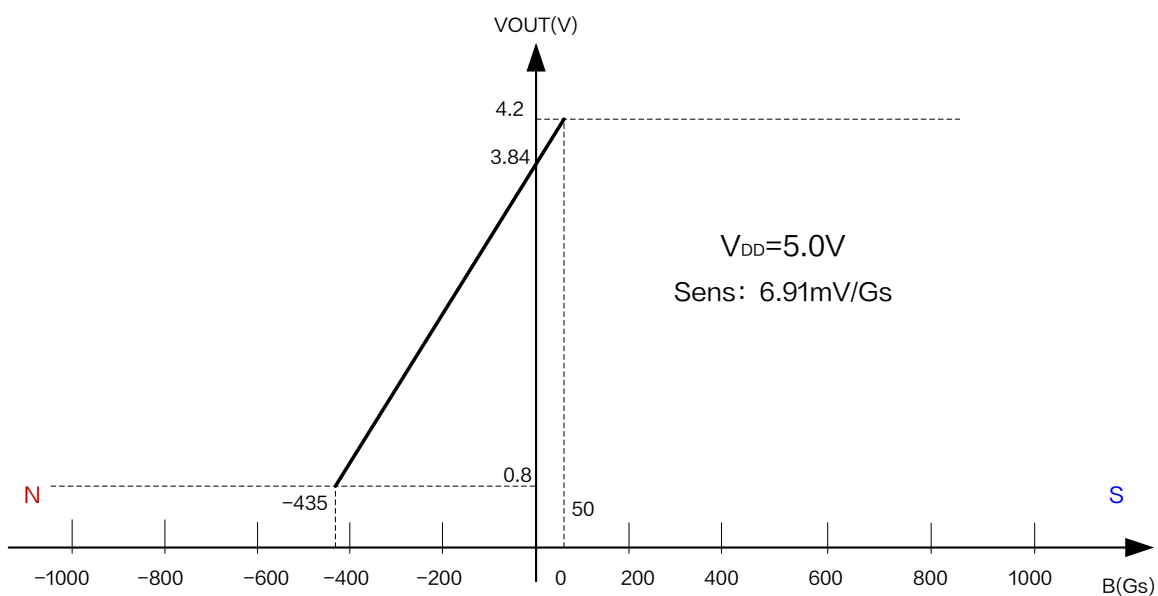
Figure6.XL48S Output characteristic curve ( V_{DD} = 5.0V )
