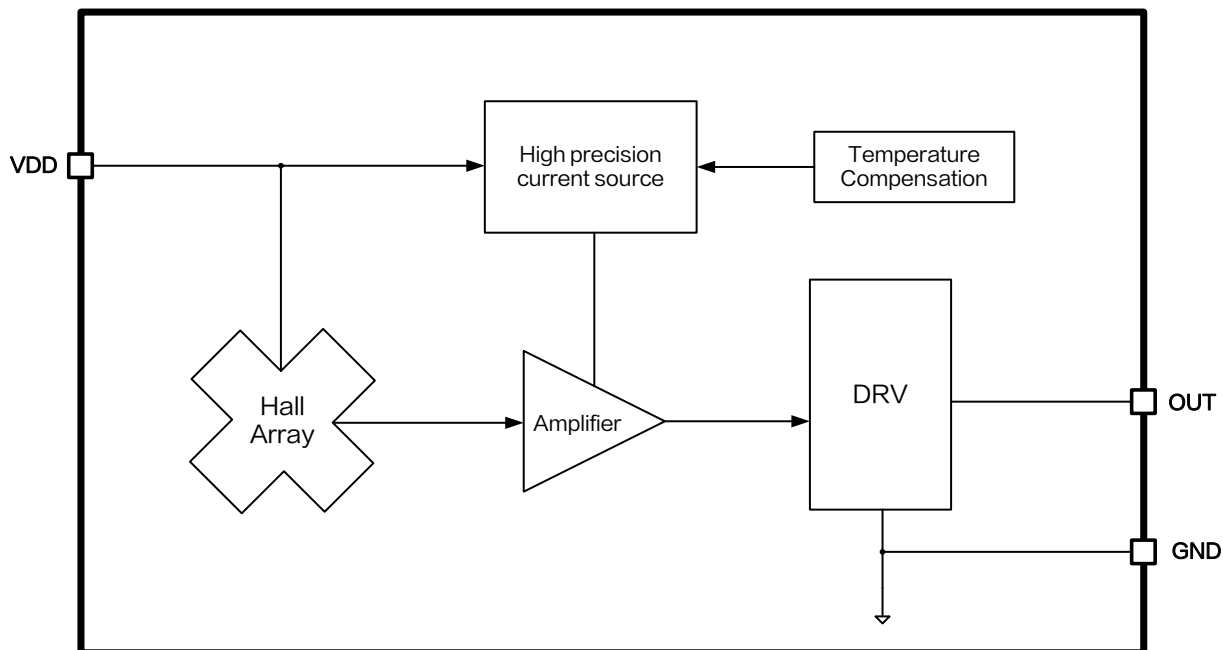
Figure3.Function Block Diagram of XL48S
