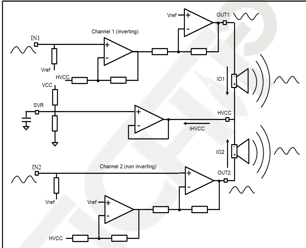
Figure 5 Amplifier Structure
