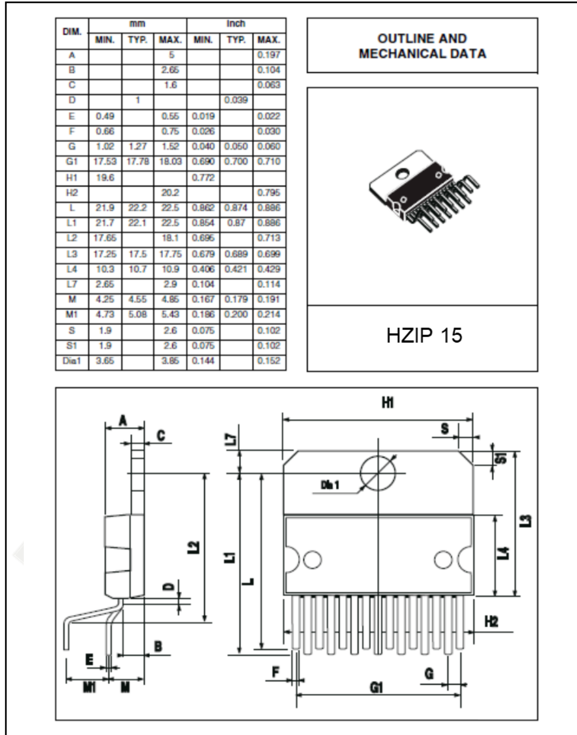
Figure 6 HZIP15 Vertical Mechanical Data and Package Dimensions
