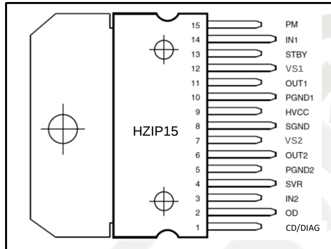
Figure 3 Pin Connection
