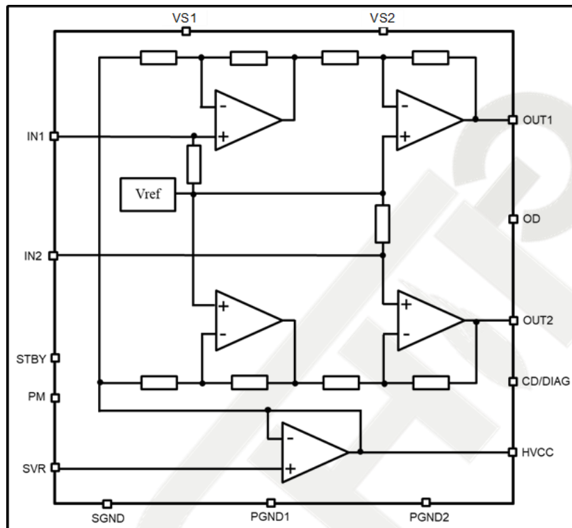
Figure 1 Block Diagram
