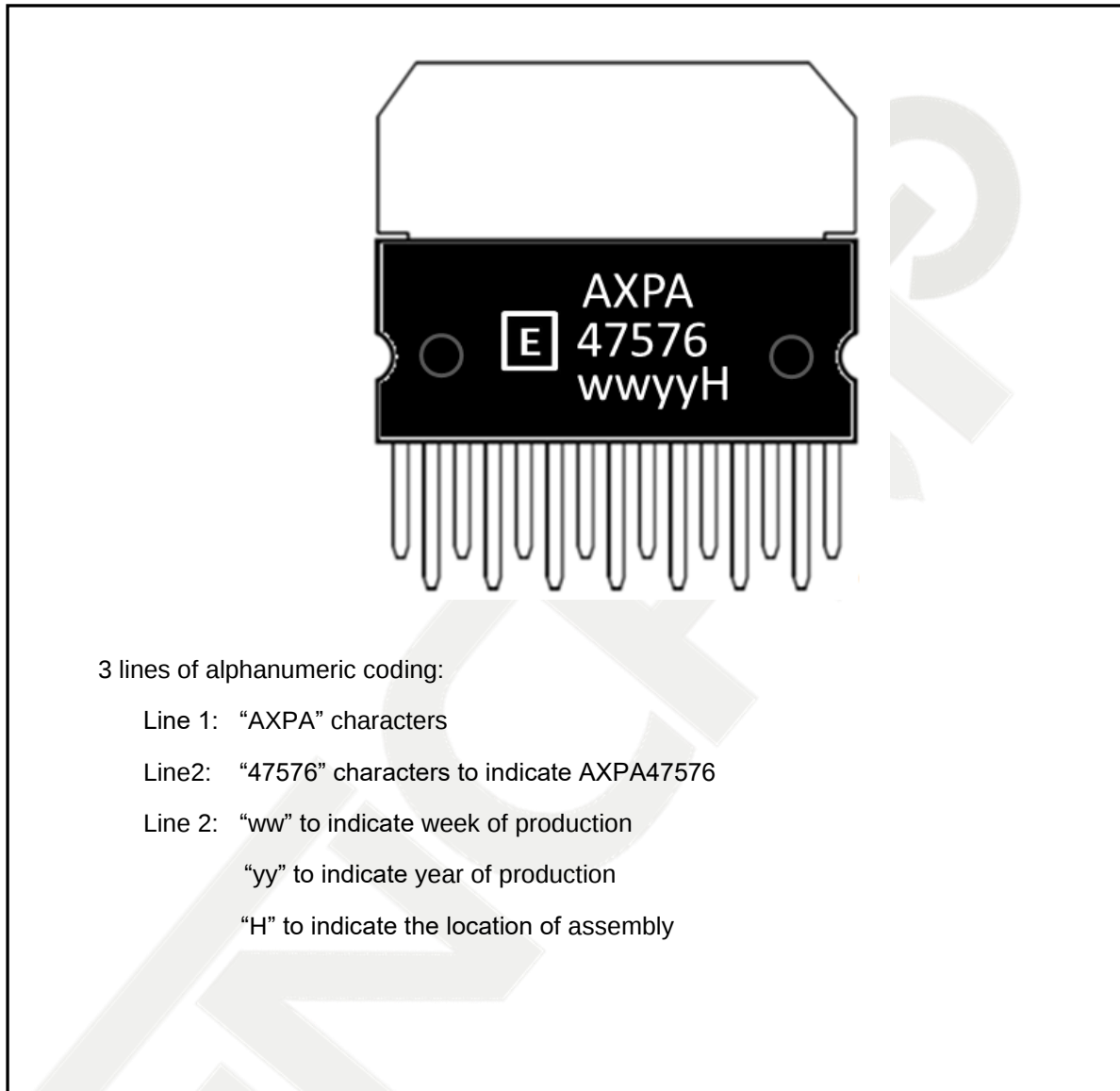
Figure 7 HZIP15 Marking Information
