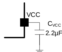
Figure 8. VCC Capacitor Connection
