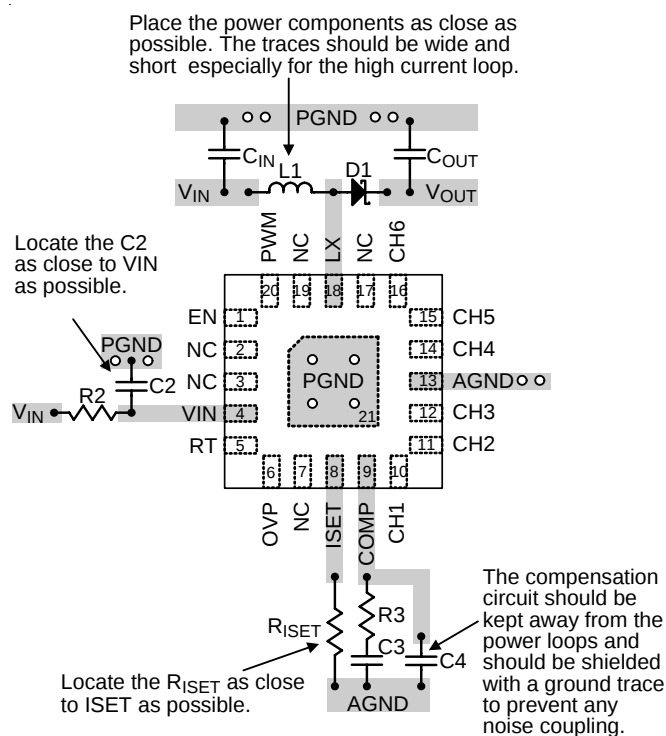
Figure 3. PCB Layout Guide
