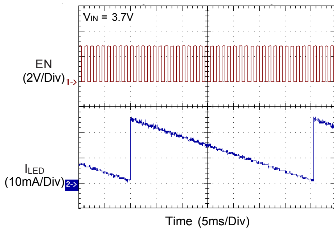
Pulse Dimming Operation
