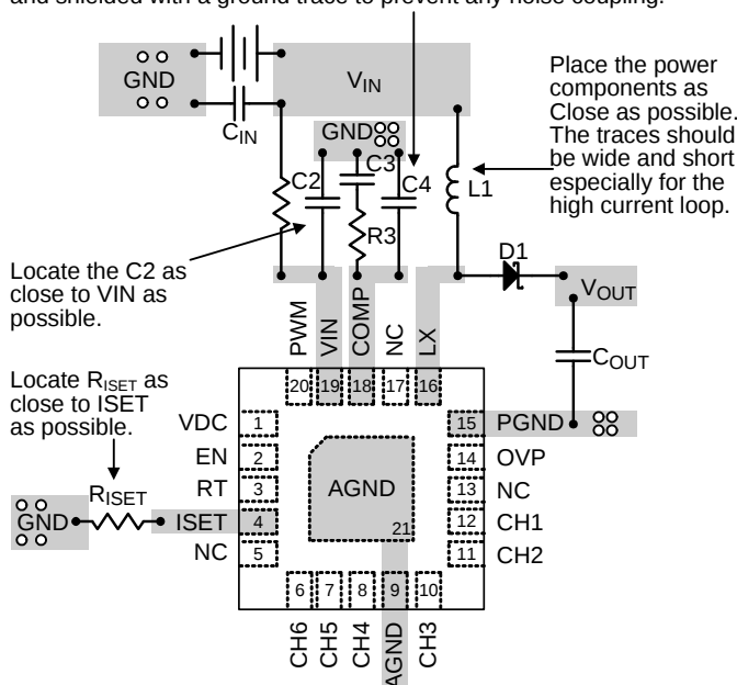
Figure 6. PCB Layout Guide
