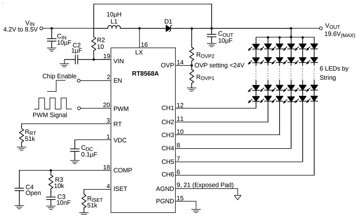
Figure 1. Application Circuit 1
