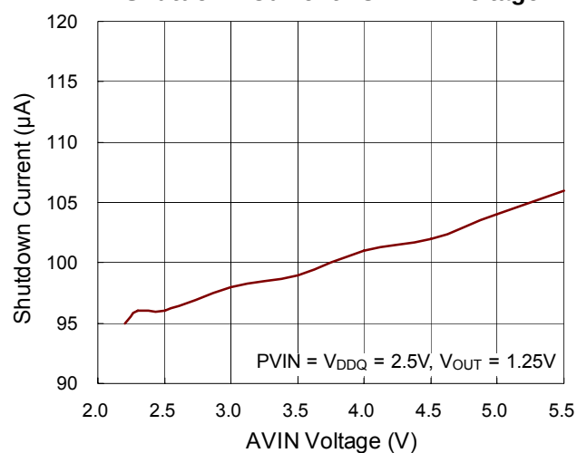
Shutdown Current vs. AVIN Voltage
