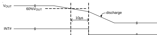
Figure 20. UVP Behavior
