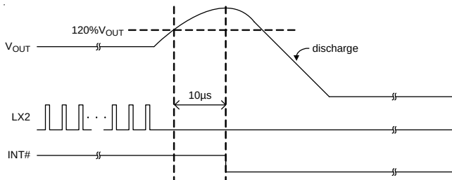
Figure 9. OVP Behavior
