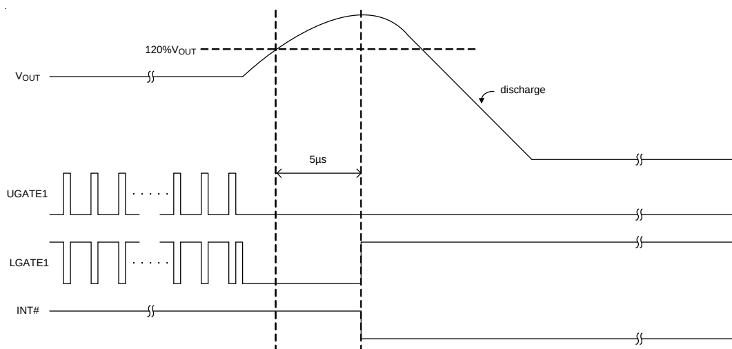
Figure 6. OVP Behavior
