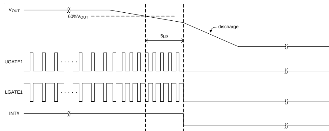
Figure 7. UVP Behavior
