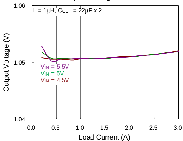
BUCK4 Output Voltage vs. Load Current
