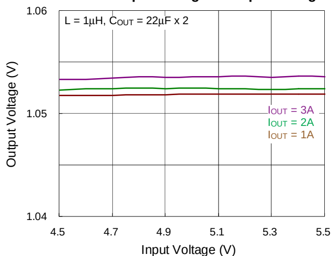
BUCK4 Output Voltage vs. Input Voltage
