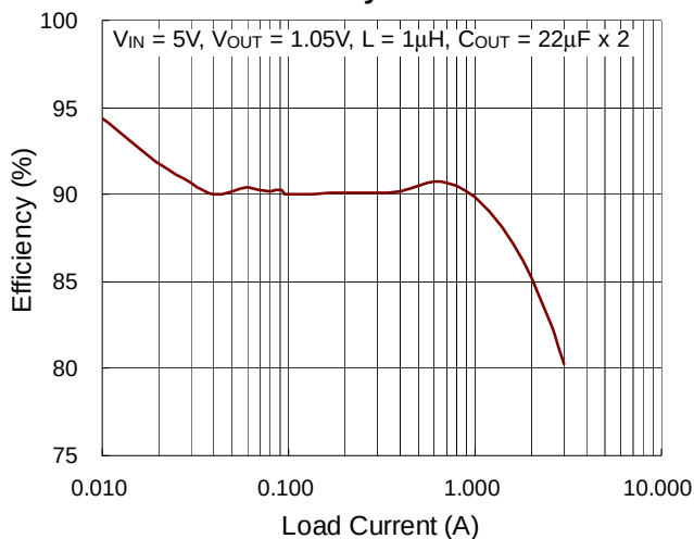
BUCK4 Efficiency vs. Load Current
