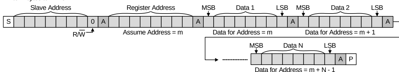
Write N bytes to PMIC
