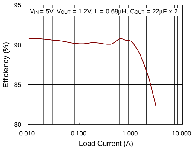
BUCK2 Efficiency vs. Load Current
