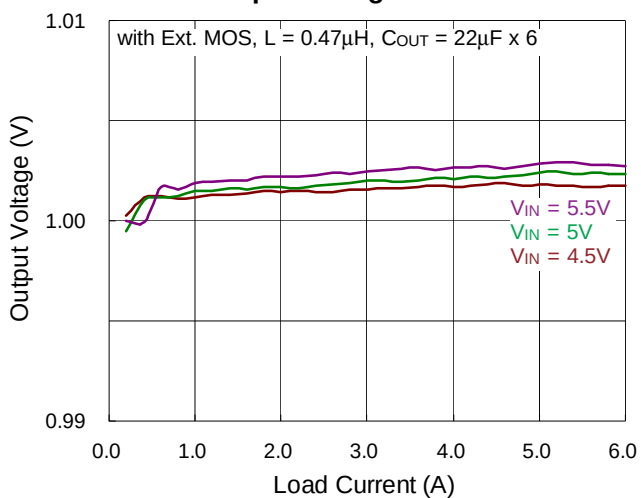
BUCK3 Output Voltage vs. Load Current
