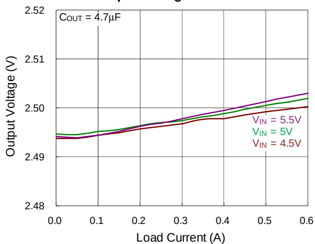
LDO Output Voltage vs. Load Current
