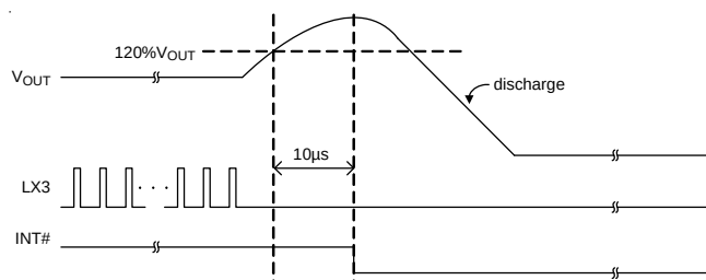
Figure 12. OVP Behavior
