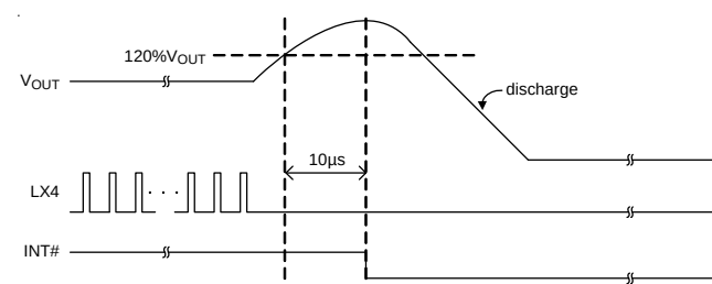
Figure 15. OVP Behavior
