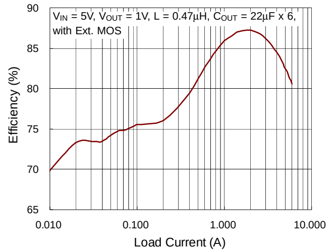
BUCK3 Efficiency vs. Load Current
