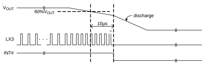
Figure 13. UVP Behavior
