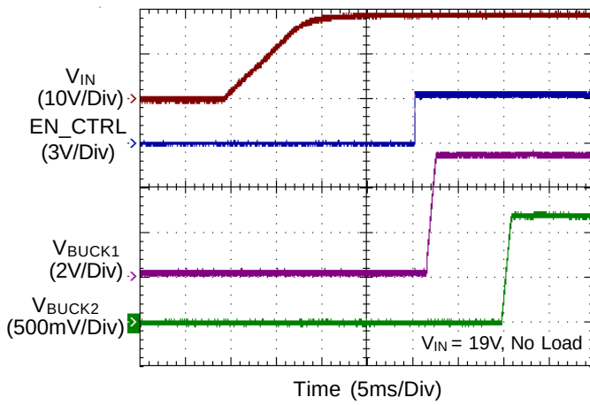
AC ON Sequence 1
