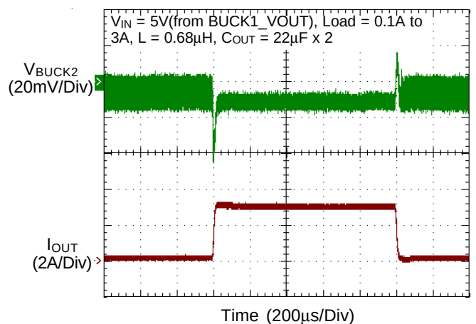
BUCK2 Load Transient
