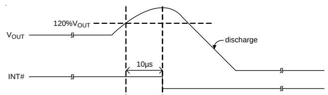
Figure 19. OVP Behavior
