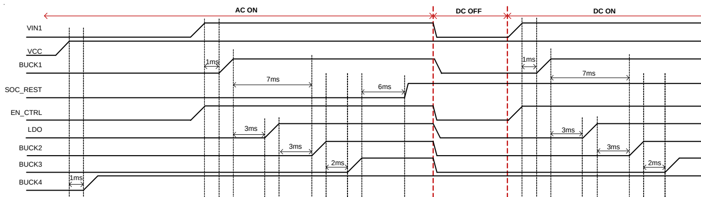
Figure 3. Power ON Sequence
