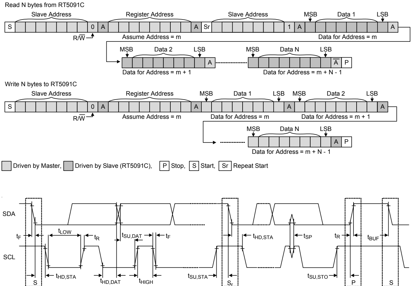
Figure 5. I 2 C Read and Write Stream and Timing Diagram
