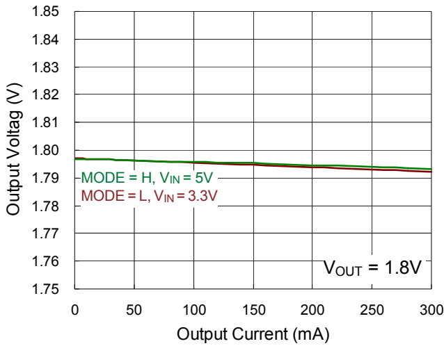
CH4 Output Voltage vs. Output Current
