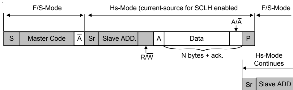
Figure 9. Data Transfer Format in Hs-Mode
