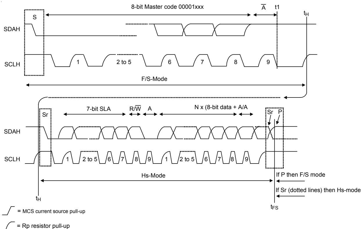
Figure 10. A Complete Hs-Mode Transfer
