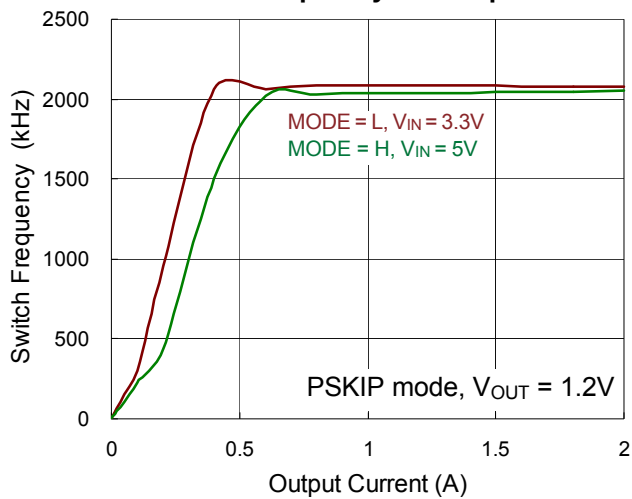
CH2 Switch Frequency vs. Output Current
