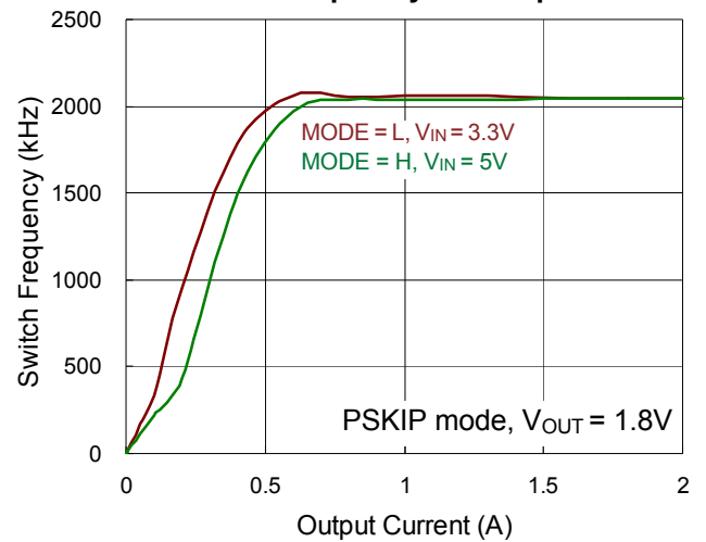
CH3 Switch Frequency vs. Output Current
