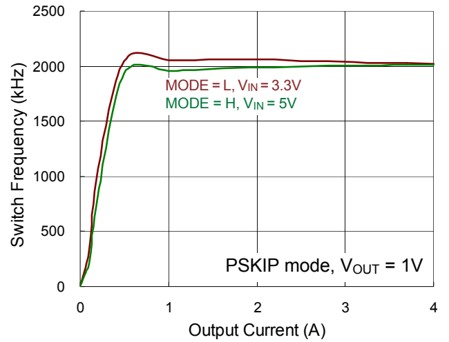
CH1 Switch Frequency vs. Output Current
