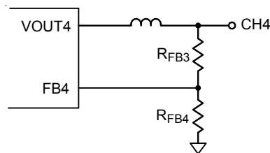
Figure 4. Setting LDO Voltage with Resistor Divider
