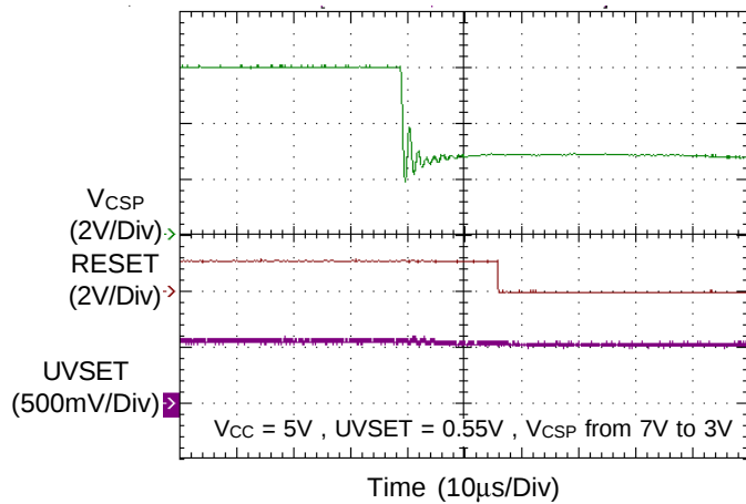
UVP vs. Reset Behavior
