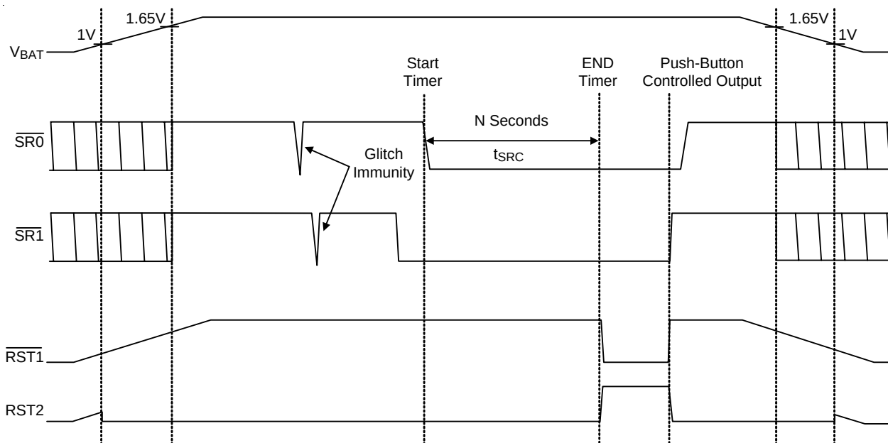
Figure 1. Timing Diagram
