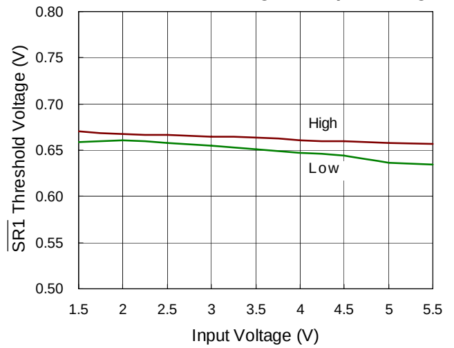
SR1 Threshold Voltage vs. Input Voltage
