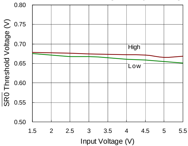
SR0 Threshold Voltage vs. Input Voltage
