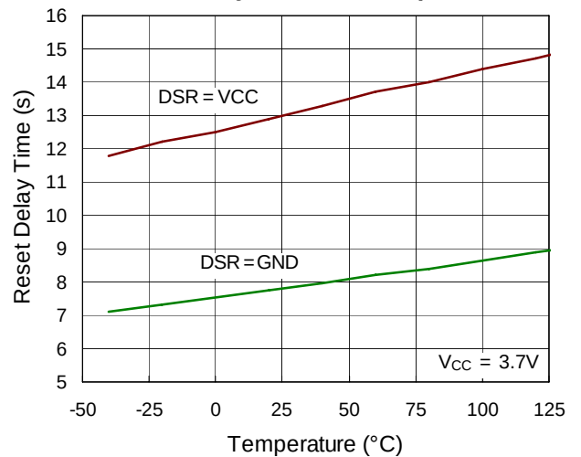
Reset Delay Time vs. Temperature
