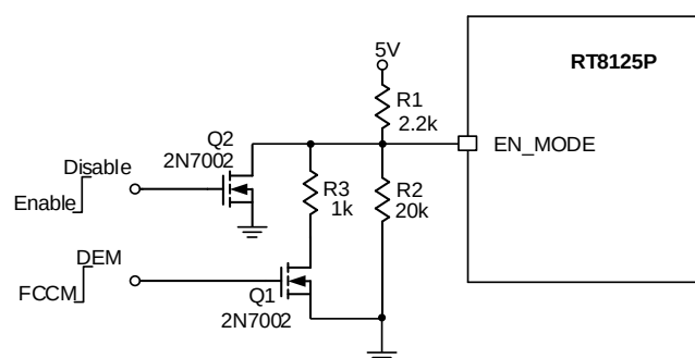
Figure 1. EN_MODE Pin Recommend Circuit
