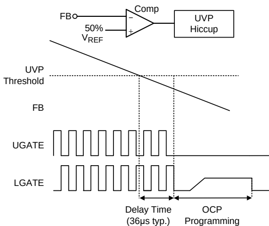
Figure 5. UVP Operation
