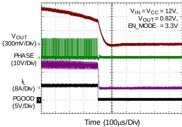
Overcurrent Limit
