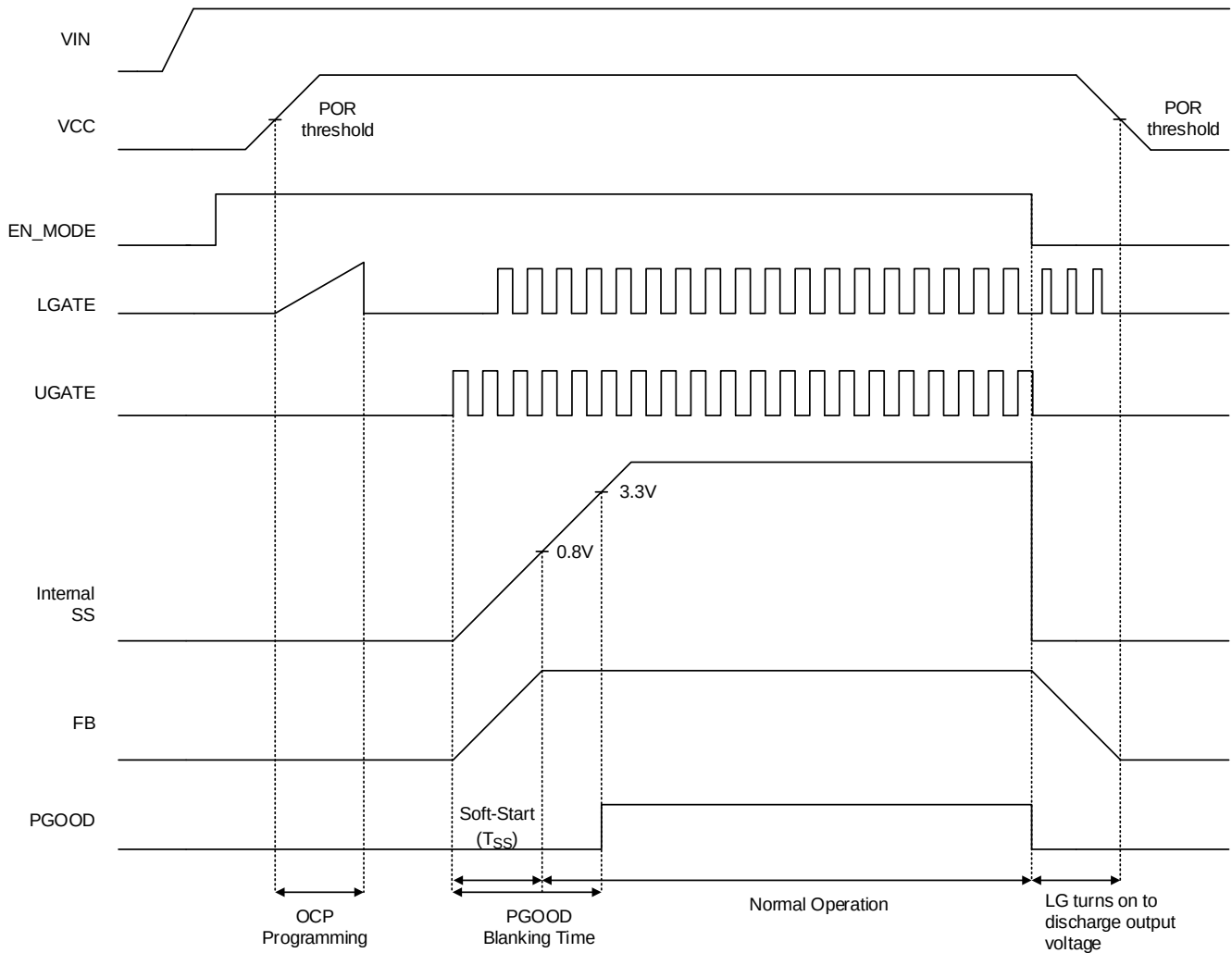
Figure 2. Soft-Start Timing Chart
