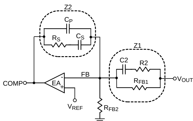
Figure 6. Type-III Compensator
