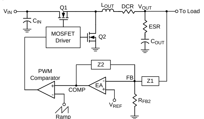
Figure 5. Voltage Mode Control Loop of Buck Converter
