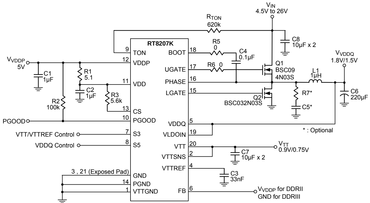
Figure 2. Fixed Voltage Regulator
