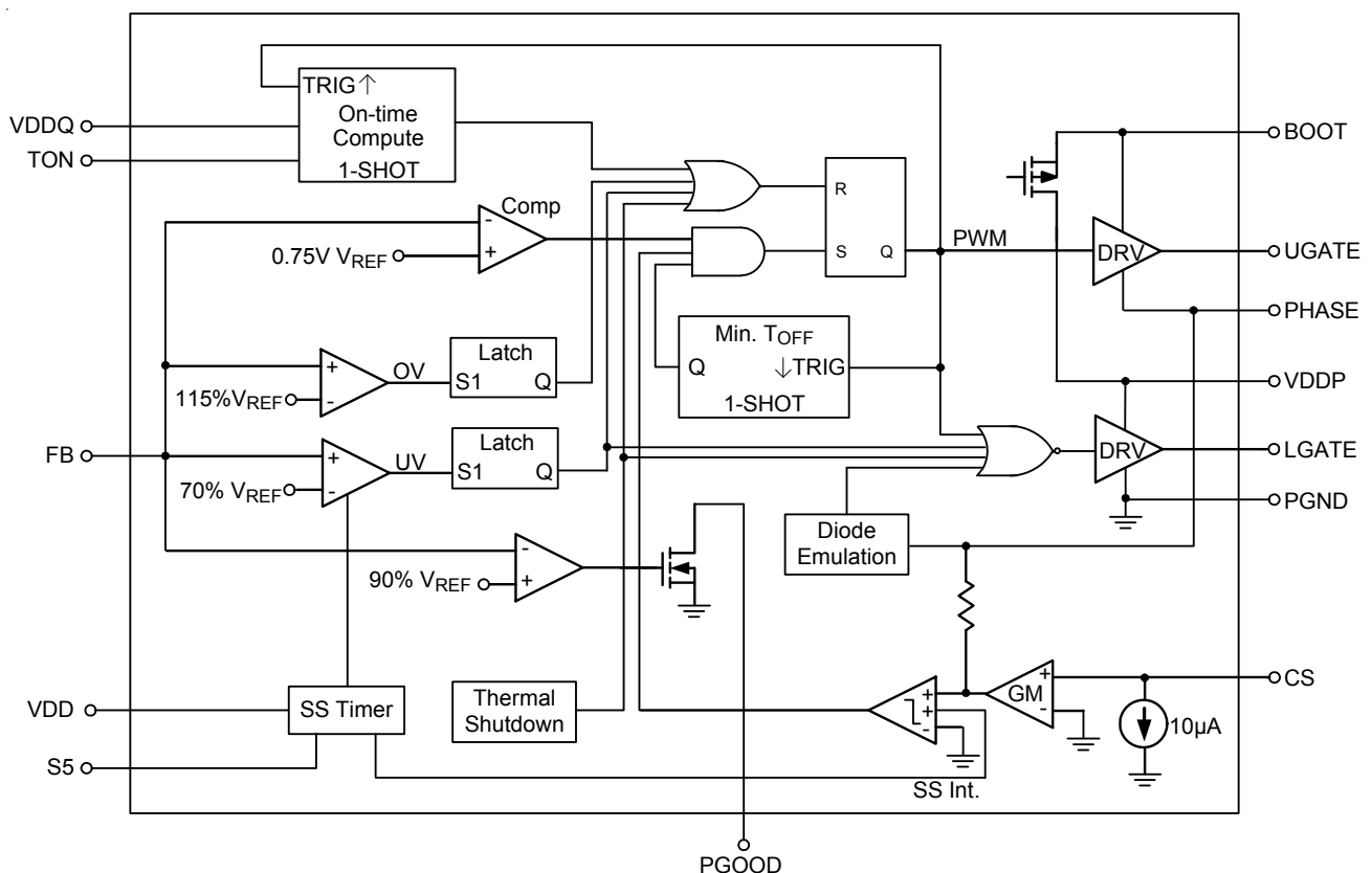
Buck Controller
