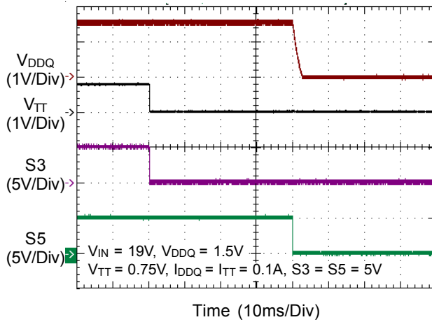
Discharge of VDDQ and VTT
