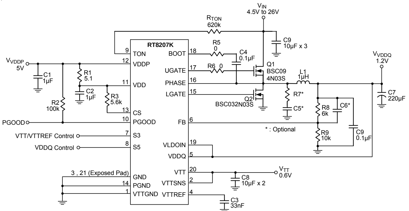
Figure 1. Adjustable Voltage Regulator
