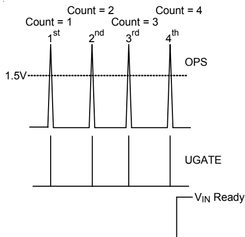
Figure 1. V_{IN} Detection Function
