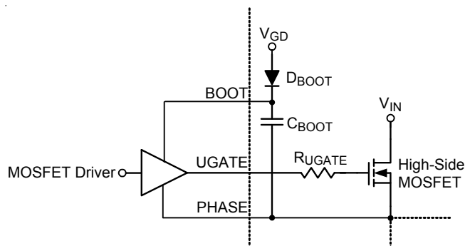
Figure 4. Bootstrap Circuit
