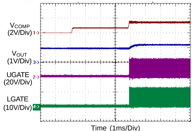
Figure 1. Power Up with Pre-Biased Output Voltage
